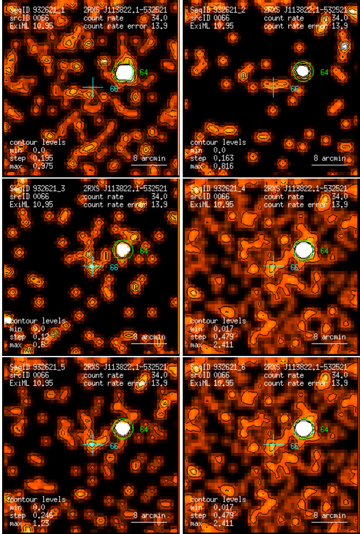
Figure 66: RASS 932621: detection 0066: band rate images, Gaussian filter: (1) PSPC channels 11 – 41, (2) 52 – 90, (3) 91 – 201, (4) 11 – 235, (5) 52 – 201, (6) 11 – 201. Broad band rates in counts/ks. Band rate contour levels in counts/ks/arcmin 2 .
