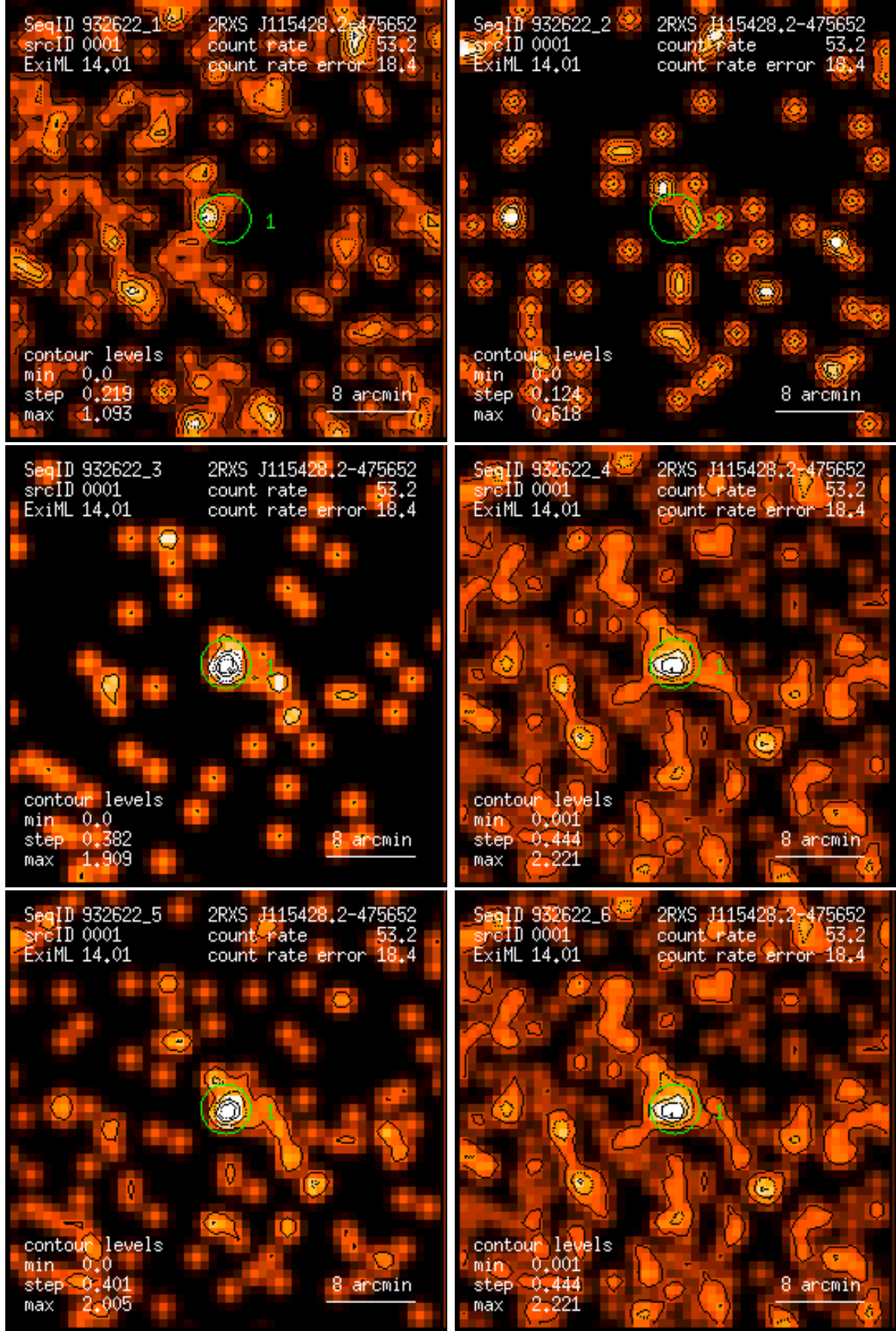
Figure 1: RASS 932622: detection 0001: band rate images, Gaussian filter: (1) PSPC channels 11 – 41, (2) 52 – 90, (3) 91 – 201, (4) 11 – 235, (5) 52 – 201, (6) 11 – 201. Broad band rates in counts/ks. Band rate contour levels in counts/ks/arcmin 2 .
