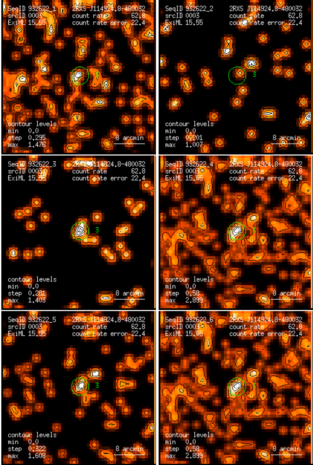
Figure 3: RASS 932622: detection 0003: band rate images, Gaussian filter: (1) PSPC channels 11 – 41, (2) 52 – 90, (3) 91 – 201, (4) 11 – 235, (5) 52 – 201, (6) 11 – 201. Broad band rates in counts/ks. Band rate contour levels in counts/ks/arcmin 2 .
