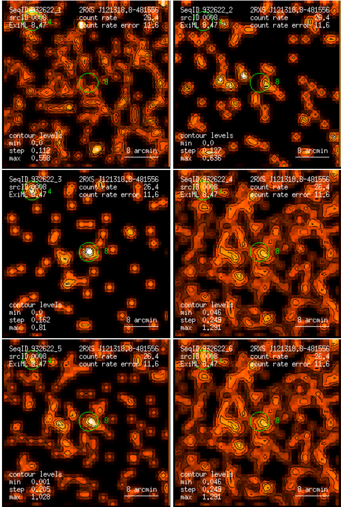
Figure 8: RASS 932622: detection 0008: band rate images, Gaussian filter: (1) PSPC channels 11 – 41, (2) 52 – 90, (3) 91 – 201, (4) 11 – 235, (5) 52 – 201, (6) 11 – 201. Broad band rates in counts/ks. Band rate contour levels in counts/ks/arcmin 2 .
