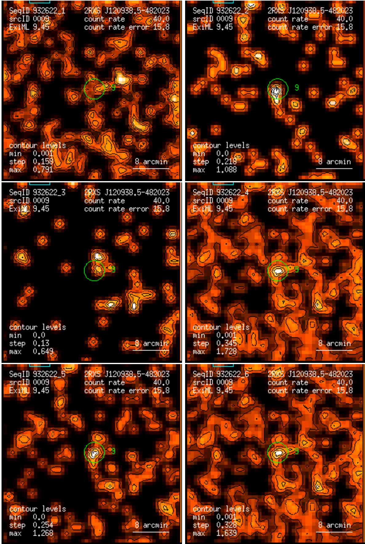
Figure 9: RASS 932622: detection 0009: band rate images, Gaussian filter: (1) PSPC channels 11 – 41, (2) 52 – 90, (3) 91 – 201, (4) 11 – 235, (5) 52 – 201, (6) 11 – 201. Broad band rates in counts/ks. Band rate contour levels in counts/ks/arcmin 2 .
