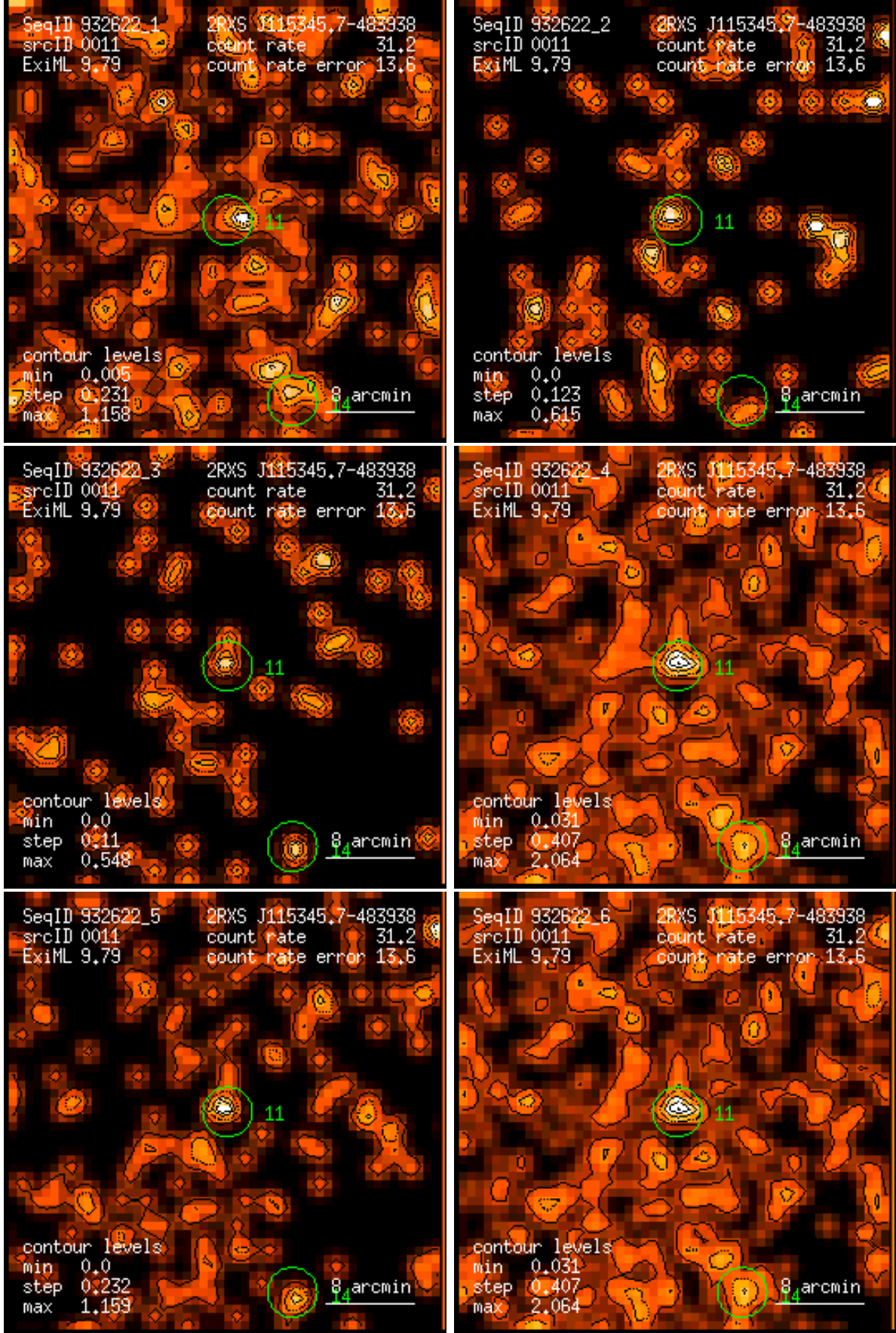
Figure 11: RASS 932622: detection 0011: band rate images, Gaussian filter: (1) PSPC channels 11 – 41, (2) 52 – 90, (3) 91 – 201, (4) 11 – 235, (5) 52 – 201, (6) 11 – 201. Broad band rates in counts/ks. Band rate contour levels in counts/ks/arcmin 2 .
