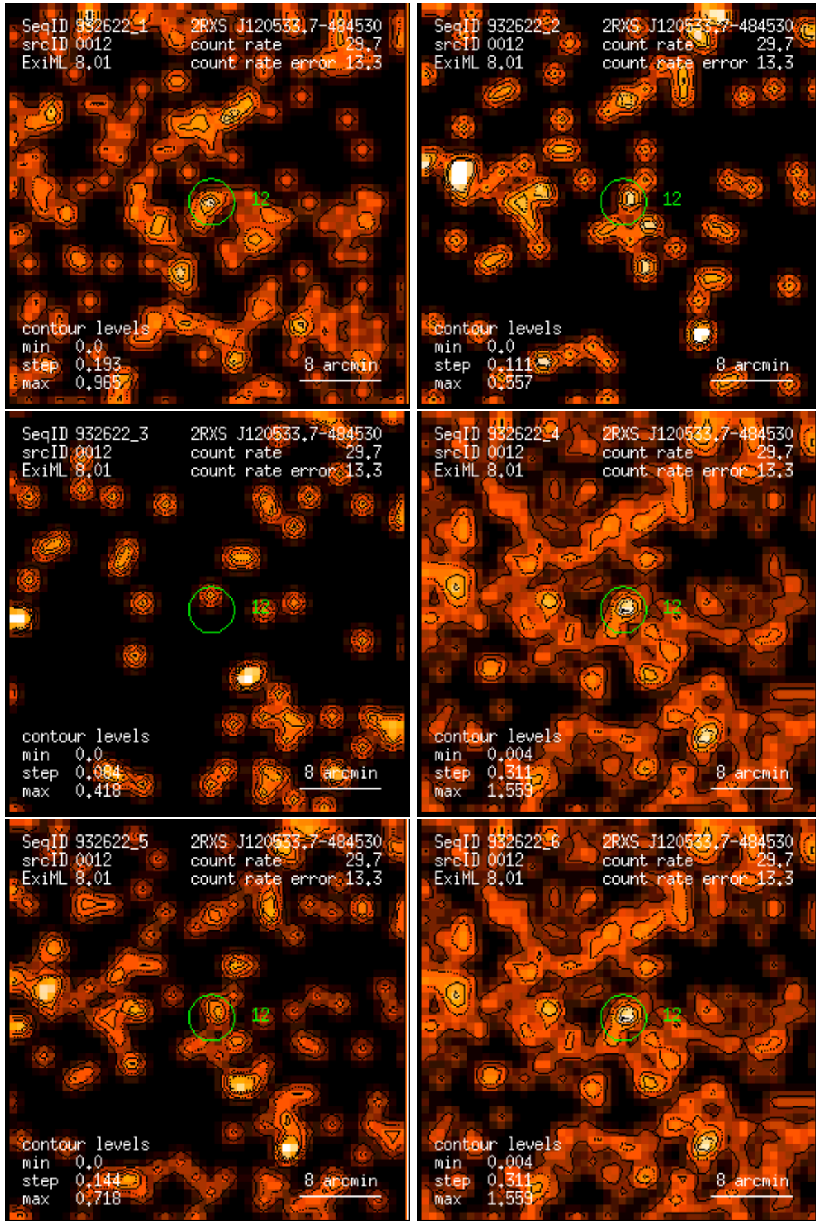
Figure 12: RASS 932622: detection 0012: band rate images, Gaussian filter: (1) PSPC channels 11 – 41, (2) 52 – 90, (3) 91 – 201, (4) 11 – 235, (5) 52 – 201, (6) 11 – 201. Broad band rates in counts/ks. Band rate contour levels in counts/ks/arcmin 2 .
