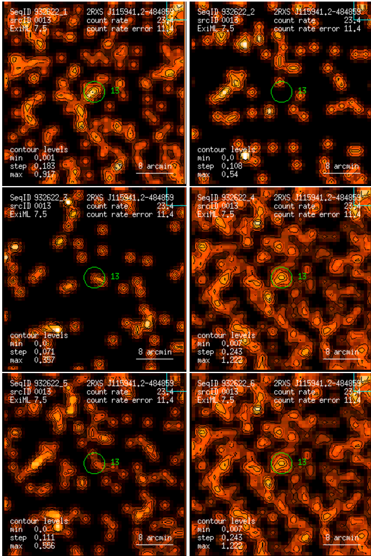
Figure 13: RASS 932622: detection 0013: band rate images, Gaussian filter: (1) PSPC channels 11 – 41, (2) 52 – 90, (3) 91 – 201, (4) 11 – 235, (5) 52 – 201, (6) 11 – 201. Broad band rates in counts/ks. Band rate contour levels in counts/ks/arcmin 2 .
