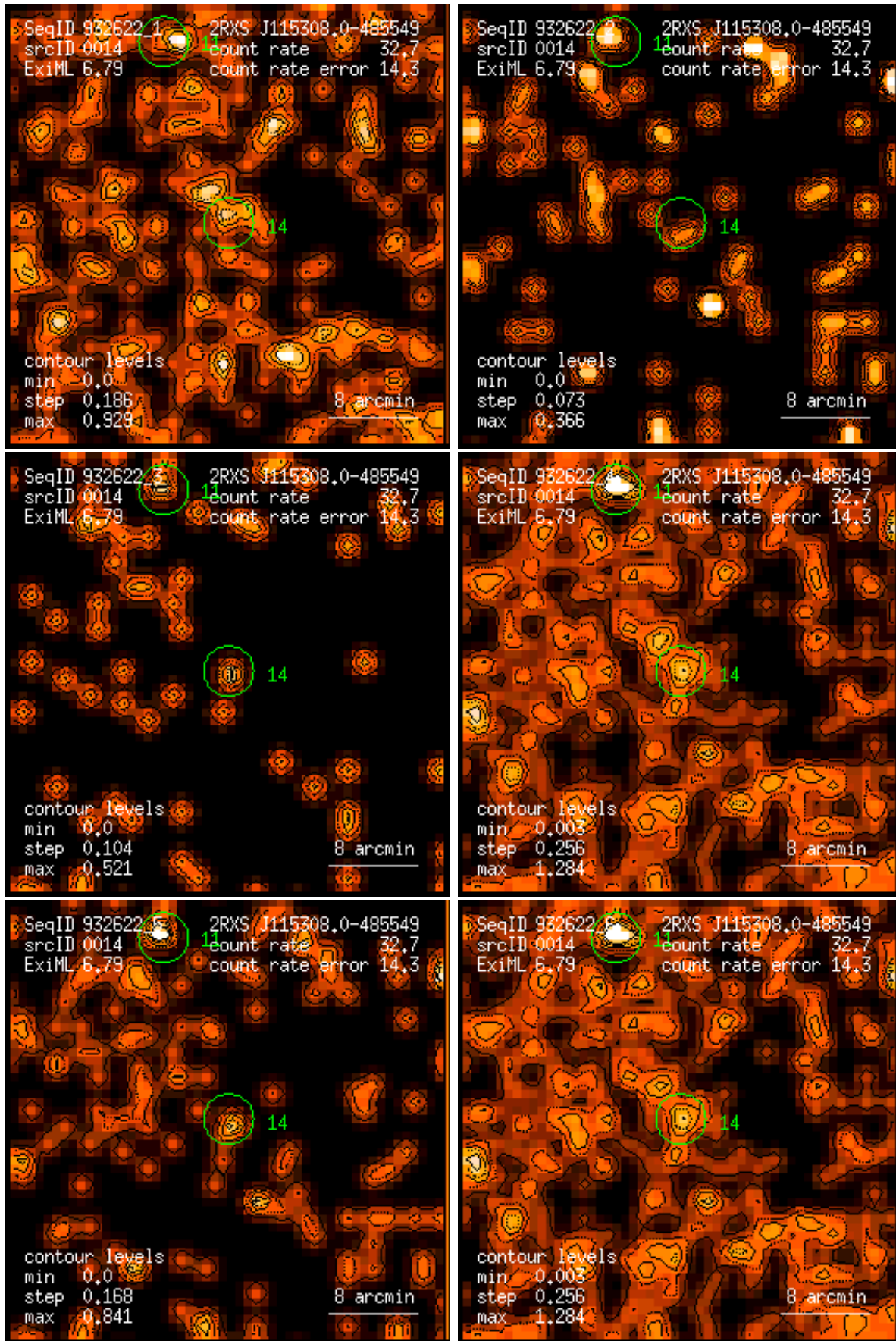
Figure 14: RASS 932622: detection 0014: band rate images, Gaussian filter: (1) PSPC channels 11 – 41, (2) 52 – 90, (3) 91 – 201, (4) 11 – 235, (5) 52 – 201, (6) 11 – 201. Broad band rates in counts/ks. Band rate contour levels in counts/ks/arcmin 2 .
