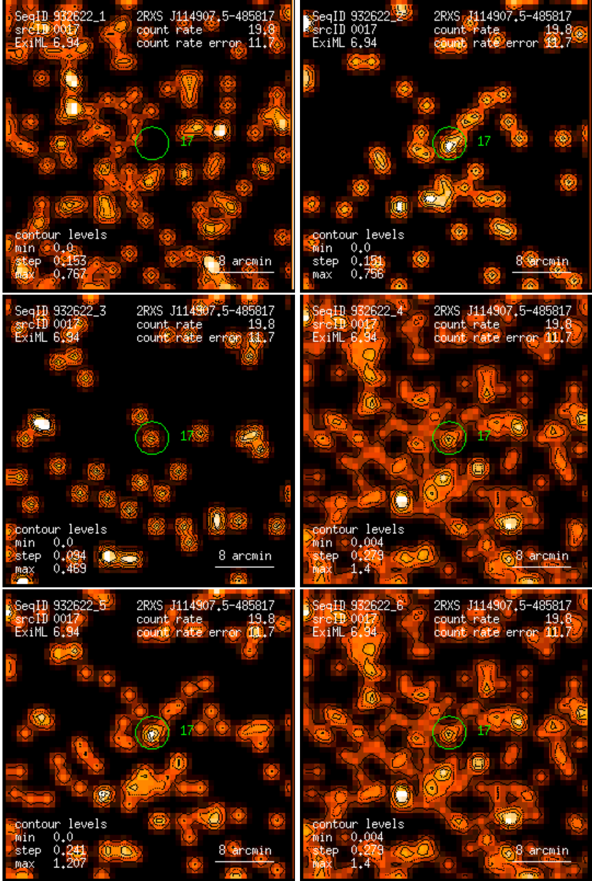
Figure 17: RASS 932622: detection 0017: band rate images, Gaussian filter: (1) PSPC channels 11 – 41, (2) 52 – 90, (3) 91 – 201, (4) 11 – 235, (5) 52 – 201, (6) 11 – 201. Broad band rates in counts/ks. Band rate contour levels in counts/ks/arcmin 2 .
