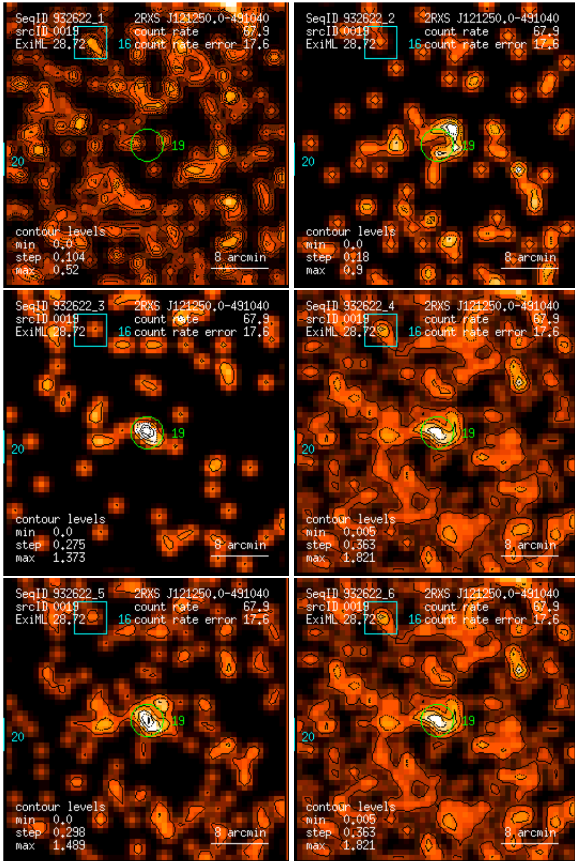
Figure 19: RASS 932622: detection 0019: band rate images, Gaussian filter: (1) PSPC channels 11 – 41, (2) 52 – 90, (3) 91 – 201, (4) 11 – 235, (5) 52 – 201, (6) 11 – 201. Broad band rates in counts/ks. Band rate contour levels in counts/ks/arcmin 2 .
