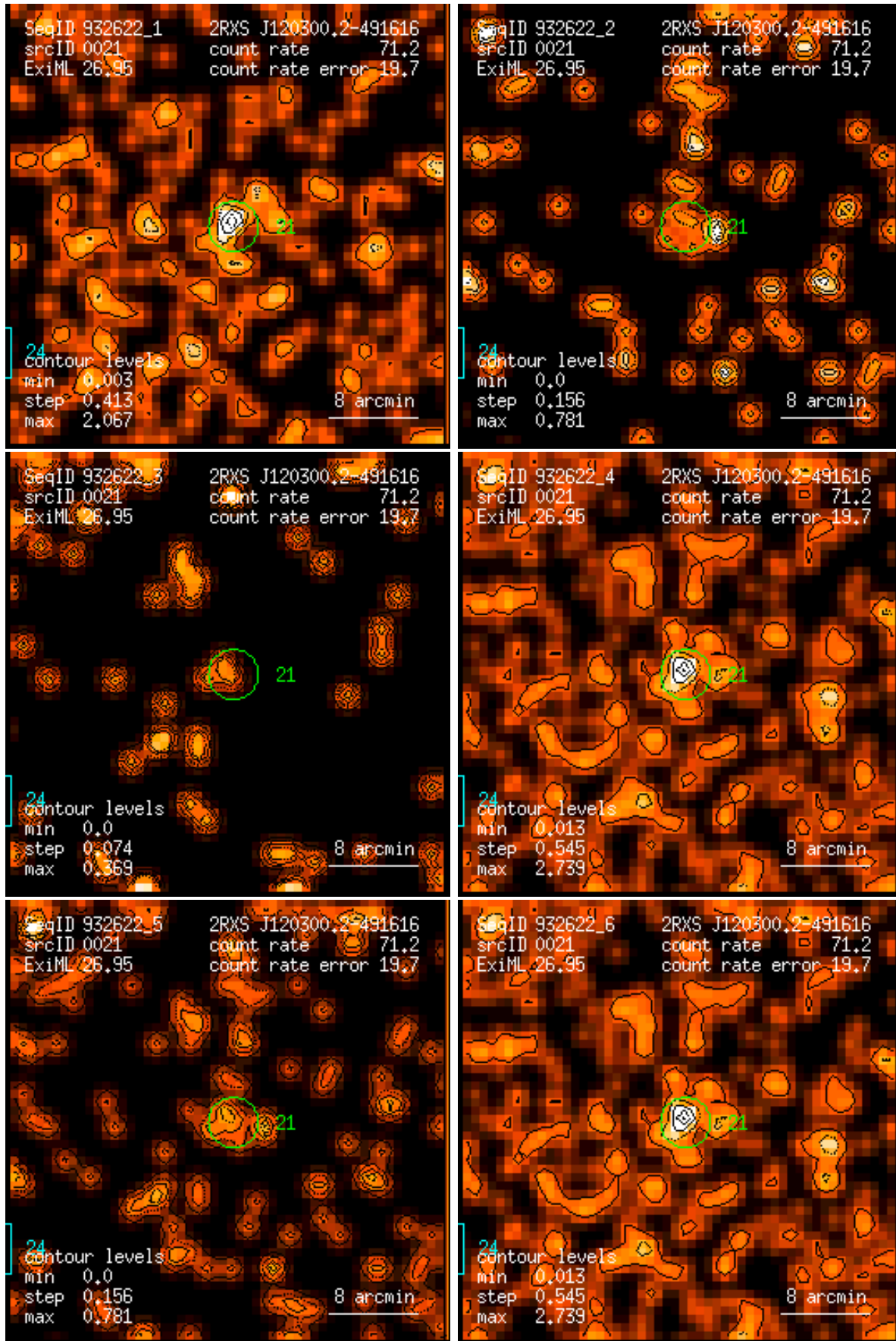
Figure 21: RASS 932622: detection 0021: band rate images, Gaussian filter: (1) PSPC channels 11 – 41, (2) 52 – 90, (3) 91 – 201, (4) 11 – 235, (5) 52 – 201, (6) 11 – 201. Broad band rates in counts/ks. Band rate contour levels in counts/ks/arcmin 2 .
