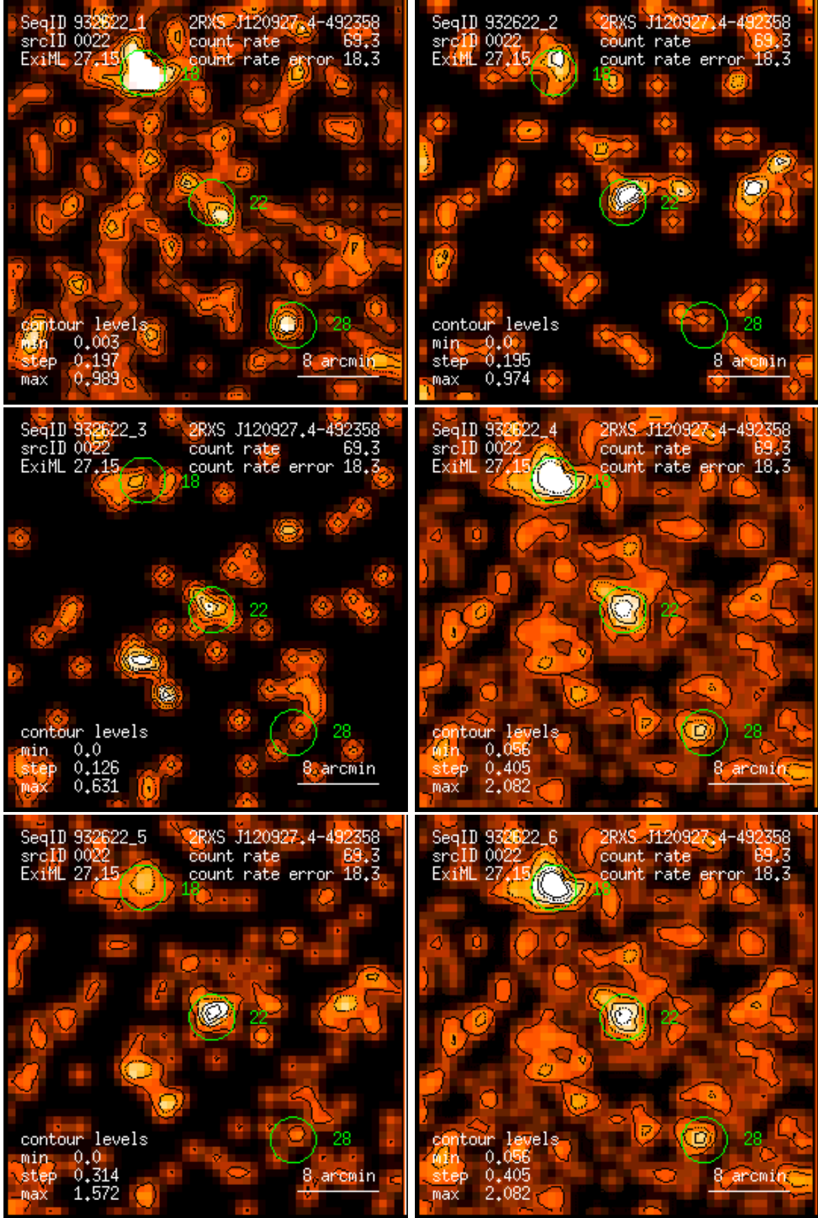
Figure 22: RASS 932622: detection 0022: band rate images, Gaussian filter: (1) PSPC channels 11 – 41, (2) 52 – 90, (3) 91 – 201, (4) 11 – 235, (5) 52 – 201, (6) 11 – 201. Broad band rates in counts/ks. Band rate contour levels in counts/ks/arcmin 2 .
