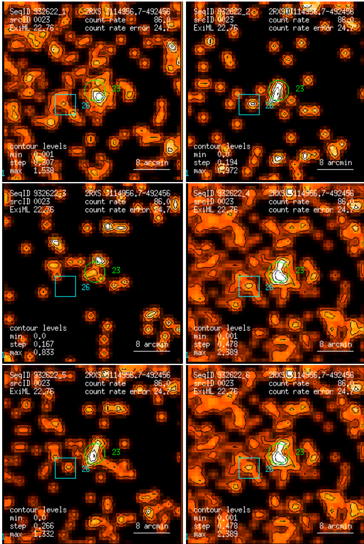
Figure 23: RASS 932622: detection 0023: band rate images, Gaussian filter: (1) PSPC channels 11 – 41, (2) 52 – 90, (3) 91 – 201, (4) 11 – 235, (5) 52 – 201, (6) 11 – 201. Broad band rates in counts/ks. Band rate contour levels in counts/ks/arcmin 2 .
