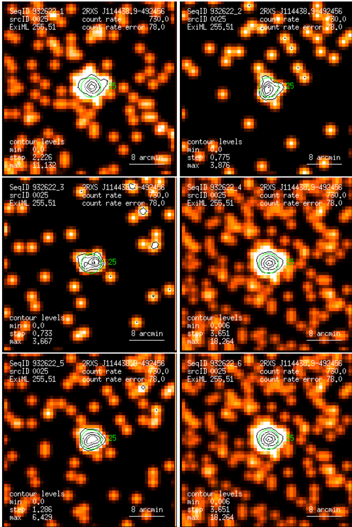
Figure 25: RASS 932622: detection 0025: band rate images, Gaussian filter: (1) PSPC channels 11 – 41, (2) 52 – 90, (3) 91 – 201, (4) 11 – 235, (5) 52 – 201, (6) 11 – 201. Broad band rates in counts/ks. Band rate contour levels in counts/ks/arcmin 2 .
