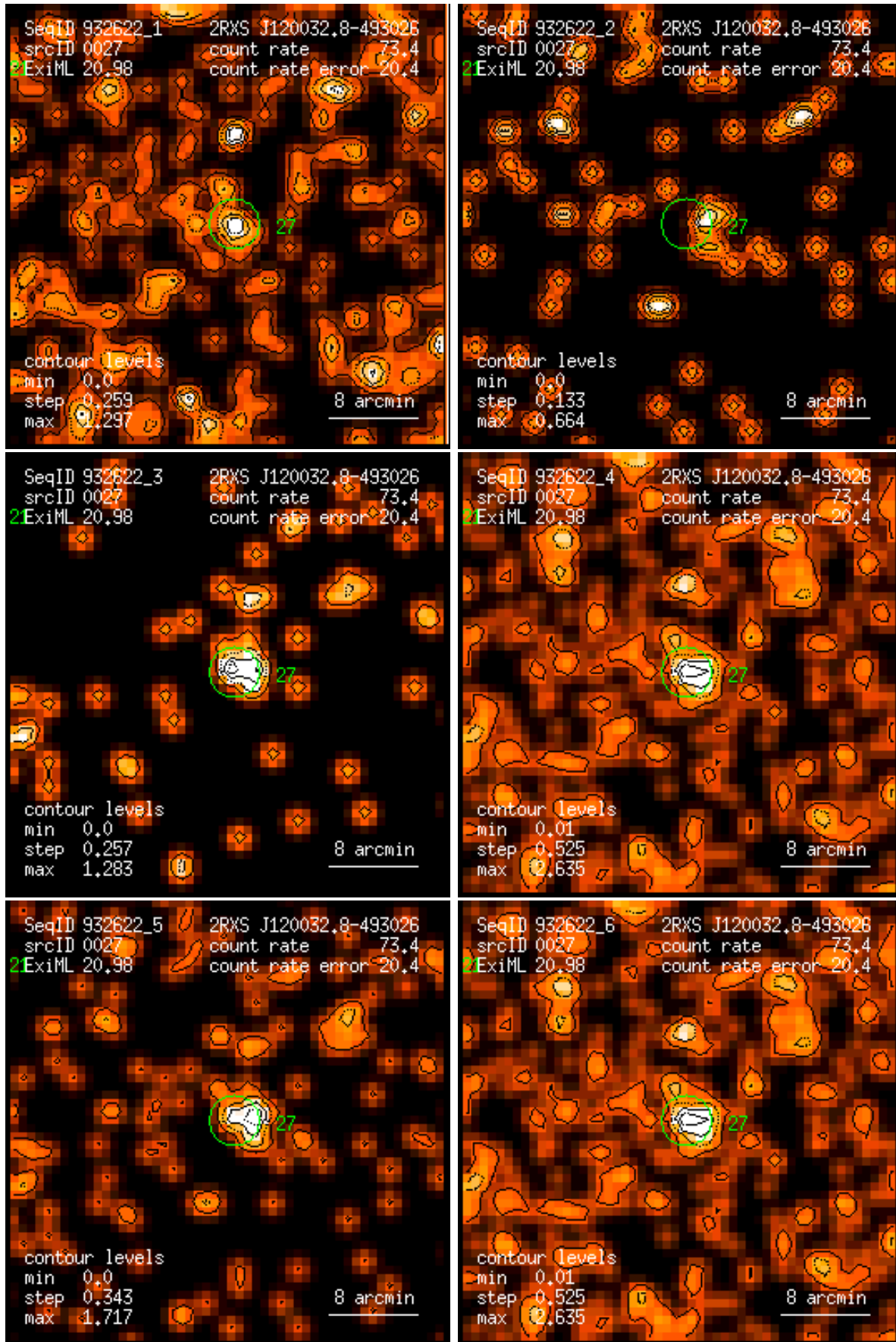
Figure 27: RASS 932622: detection 0027: band rate images, Gaussian filter: (1) PSPC channels 11 – 41, (2) 52 – 90, (3) 91 – 201, (4) 11 – 235, (5) 52 – 201, (6) 11 – 201. Broad band rates in counts/ks. Band rate contour levels in counts/ks/arcmin 2 .
