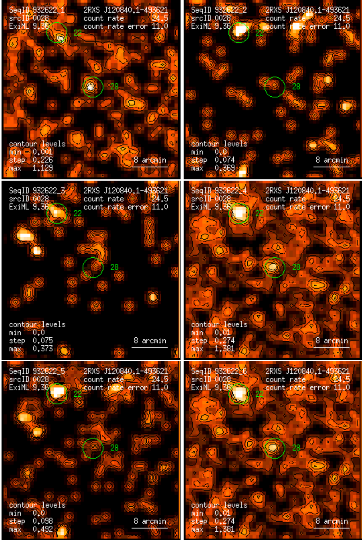
Figure 28: RASS 932622: detection 0028: band rate images, Gaussian filter: (1) PSPC channels 11 – 41, (2) 52 – 90, (3) 91 – 201, (4) 11 – 235, (5) 52 – 201, (6) 11 – 201. Broad band rates in counts/ks. Band rate contour levels in counts/ks/arcmin 2 .
