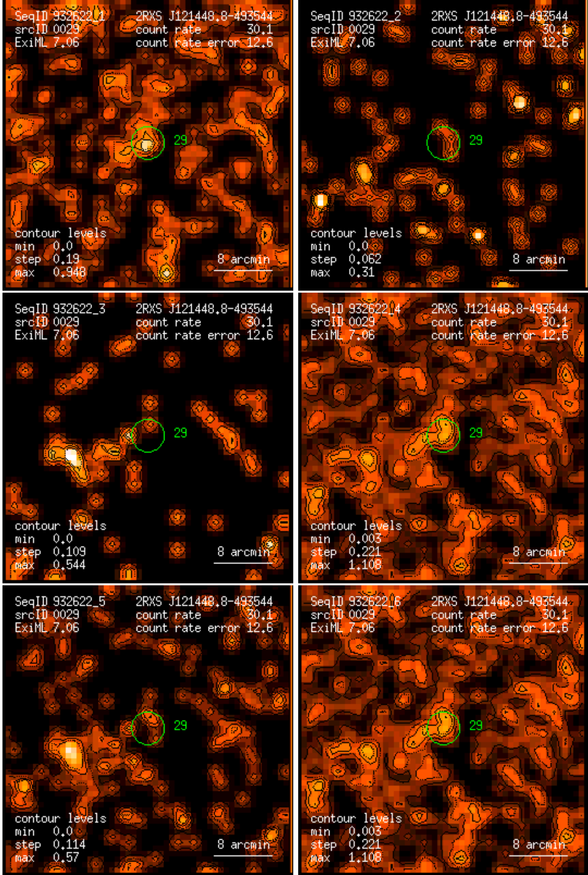
Figure 29: RASS 932622: detection 0029: band rate images, Gaussian filter: (1) PSPC channels 11 – 41, (2) 52 – 90, (3) 91 – 201, (4) 11 – 235, (5) 52 – 201, (6) 11 – 201. Broad band rates in counts/ks. Band rate contour levels in counts/ks/arcmin 2 .
