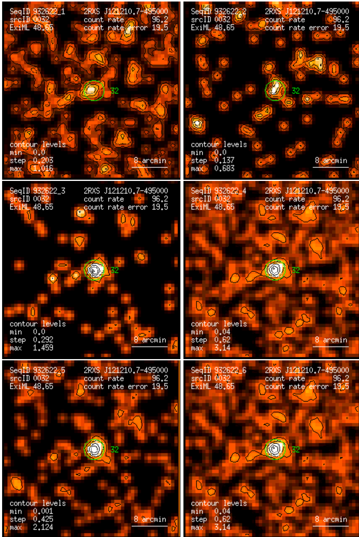
Figure 32: RASS 932622: detection 0032: band rate images, Gaussian filter: (1) PSPC channels 11 – 41, (2) 52 – 90, (3) 91 – 201, (4) 11 – 235, (5) 52 – 201, (6) 11 – 201. Broad band rates in counts/ks. Band rate contour levels in counts/ks/arcmin 2 .
