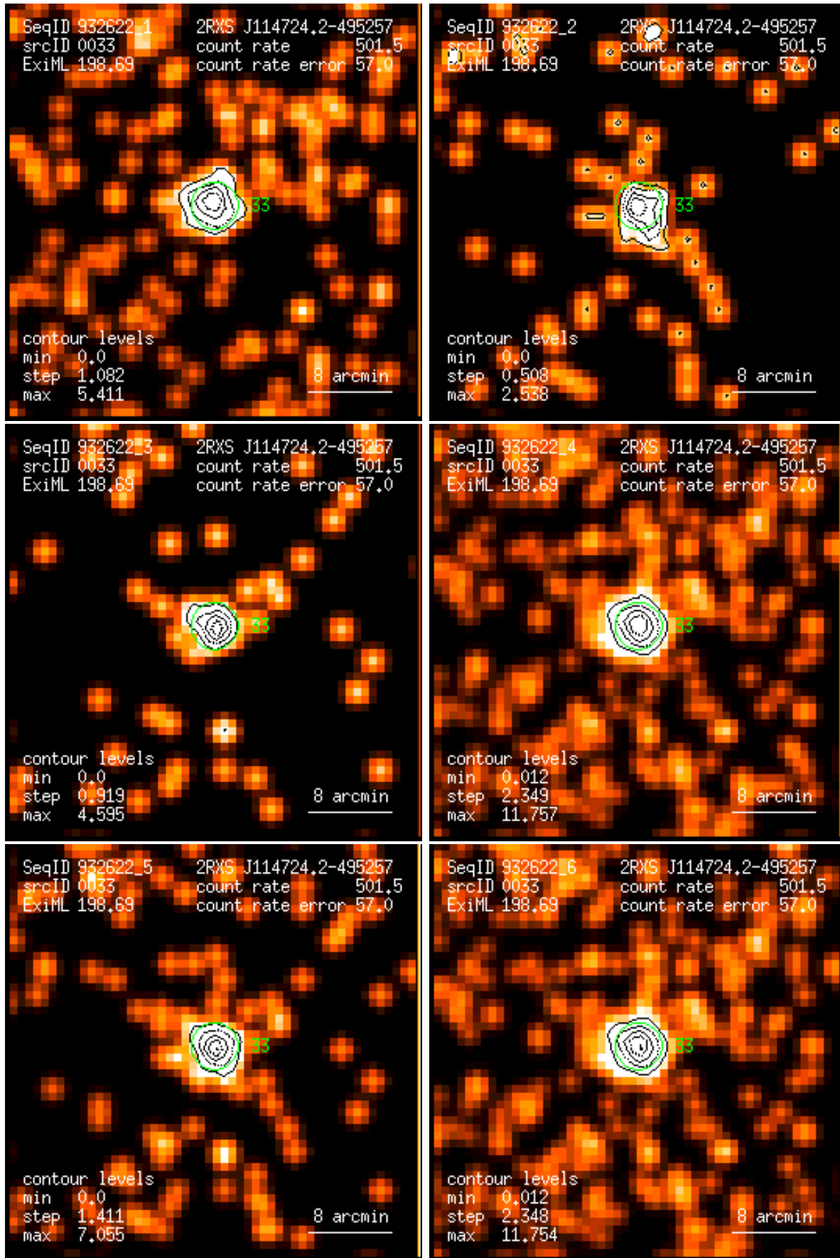
Figure 33: RASS 932622: detection 0033: band rate images, Gaussian filter: (1) PSPC channels 11 – 41, (2) 52 – 90, (3) 91 – 201, (4) 11 – 235, (5) 52 – 201, (6) 11 – 201. Broad band rates in counts/ks. Band rate contour levels in counts/ks/arcmin 2 .
