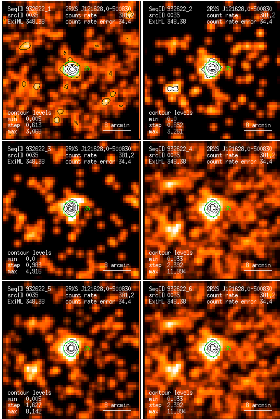
Figure 35: RASS 932622: detection 0035: band rate images, Gaussian filter: (1) PSPC channels 11 – 41, (2) 52 – 90, (3) 91 – 201, (4) 11 – 235, (5) 52 – 201, (6) 11 – 201. Broad band rates in counts/ks. Band rate contour levels in counts/ks/arcmin 2 .
