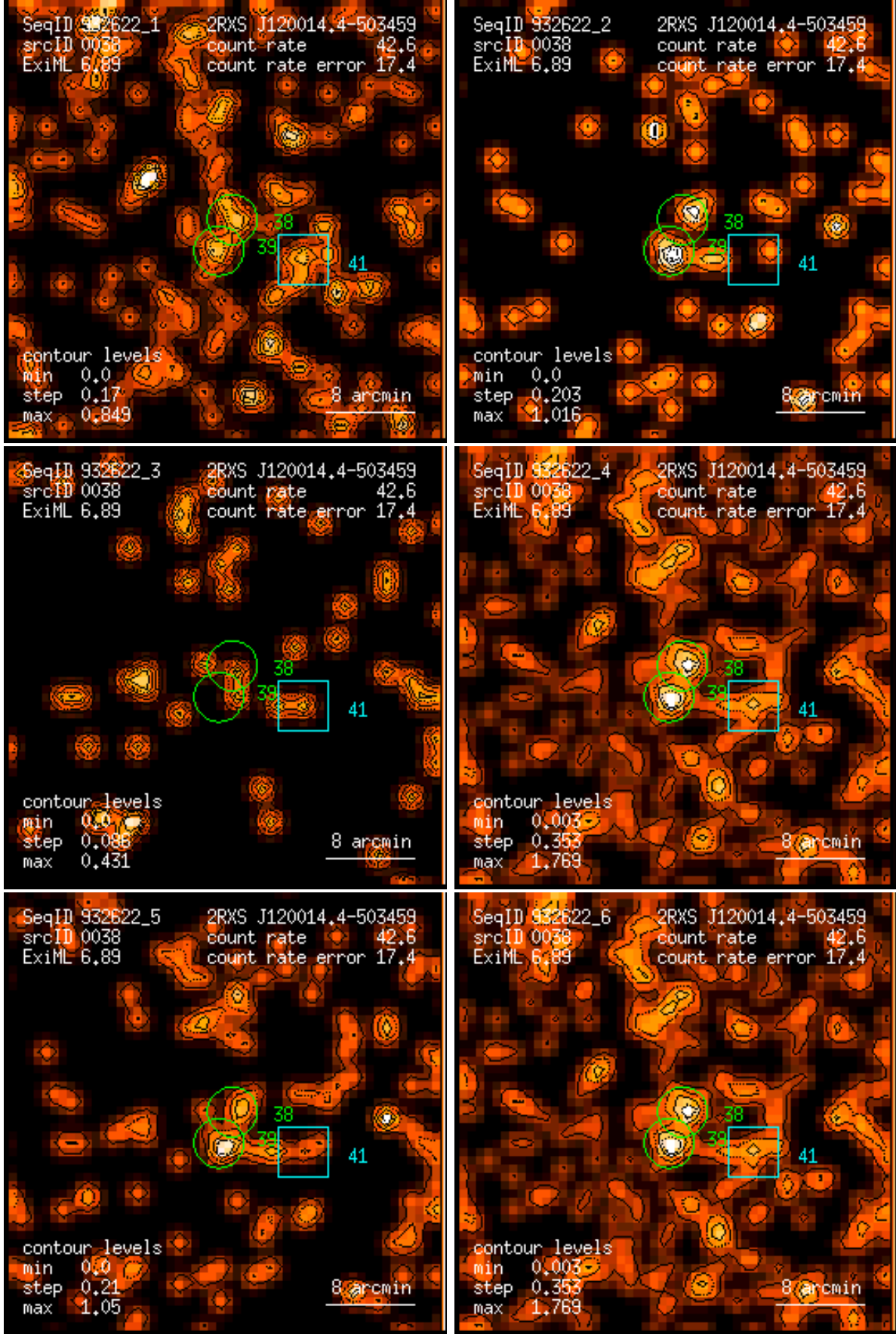
Figure 38: RASS 932622: detection 0038: band rate images, Gaussian filter: (1) PSPC channels 11 – 41, (2) 52 – 90, (3) 91 – 201, (4) 11 – 235, (5) 52 – 201, (6) 11 – 201. Broad band rates in counts/ks. Band rate contour levels in counts/ks/arcmin 2 .
