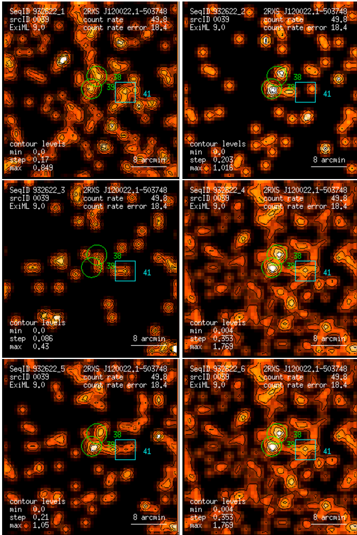
Figure 39: RASS 932622: detection 0039: band rate images, Gaussian filter: (1) PSPC channels 11 – 41, (2) 52 – 90, (3) 91 – 201, (4) 11 – 235, (5) 52 – 201, (6) 11 – 201. Broad band rates in counts/ks. Band rate contour levels in counts/ks/arcmin 2 .
