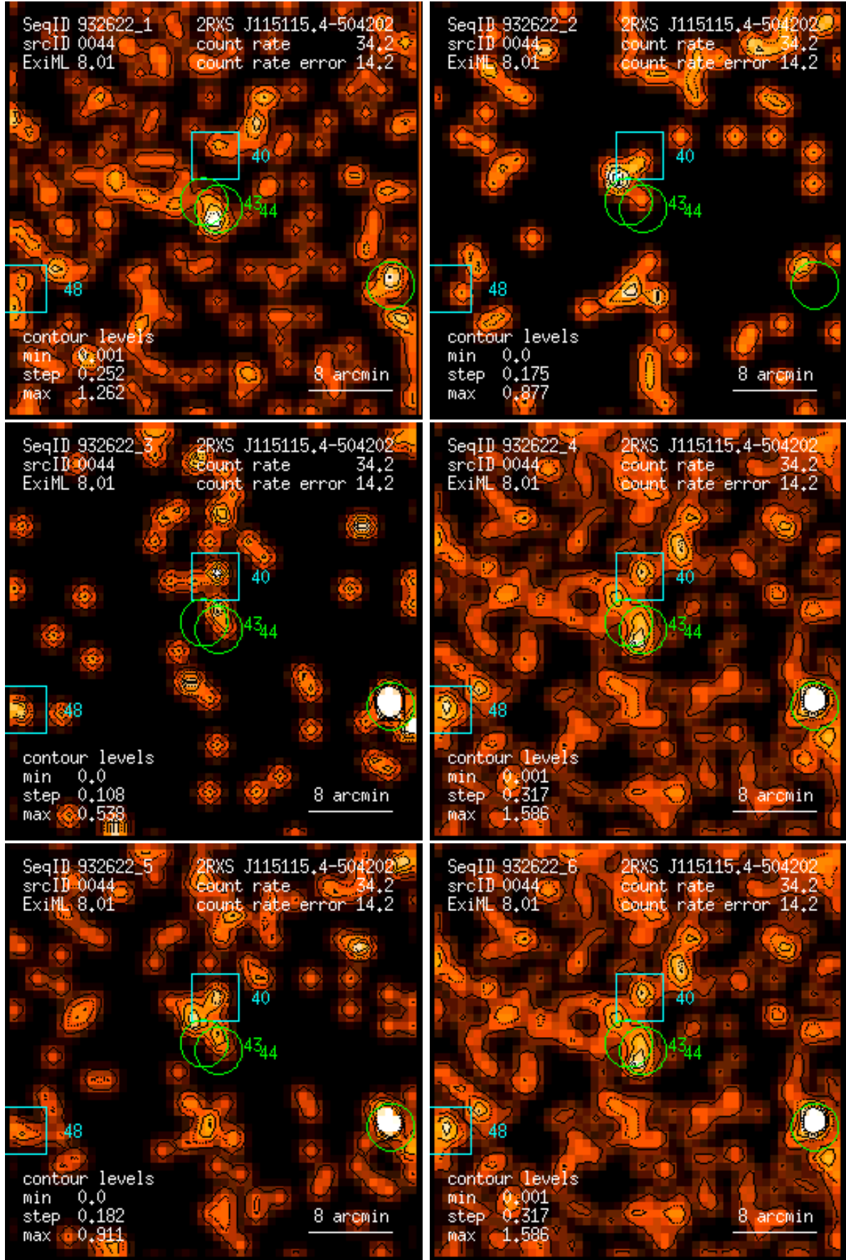
Figure 44: RASS 932622: detection 0044: band rate images, Gaussian filter: (1) PSPC channels 11 – 41, (2) 52 – 90, (3) 91 – 201, (4) 11 – 235, (5) 52 – 201, (6) 11 – 201. Broad band rates in counts/ks. Band rate contour levels in counts/ks/arcmin 2 .
