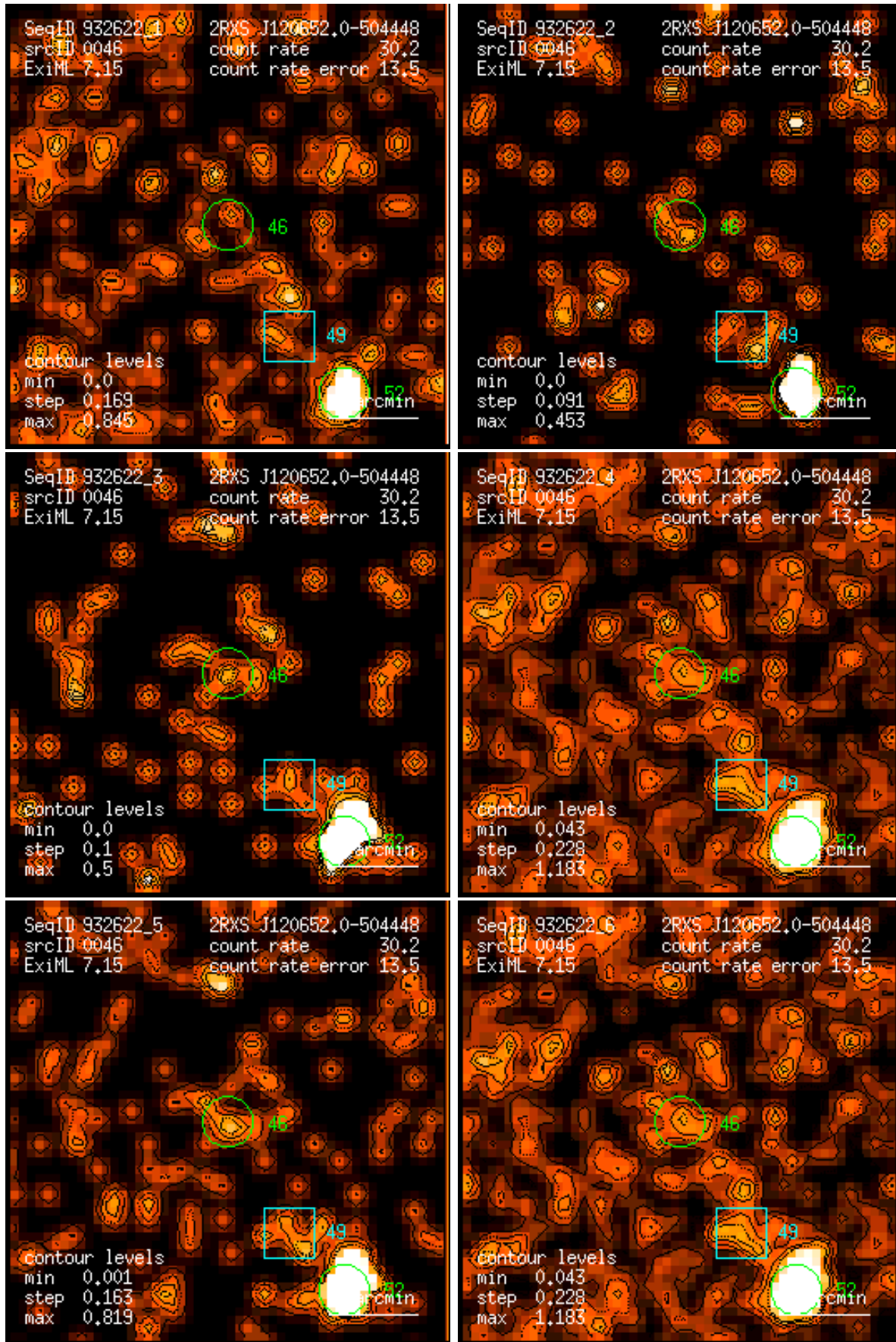
Figure 46: RASS 932622: detection 0046: band rate images, Gaussian filter: (1) PSPC channels 11 – 41, (2) 52 – 90, (3) 91 – 201, (4) 11 – 235, (5) 52 – 201, (6) 11 – 201. Broad band rates in counts/ks. Band rate contour levels in counts/ks/arcmin 2 .
