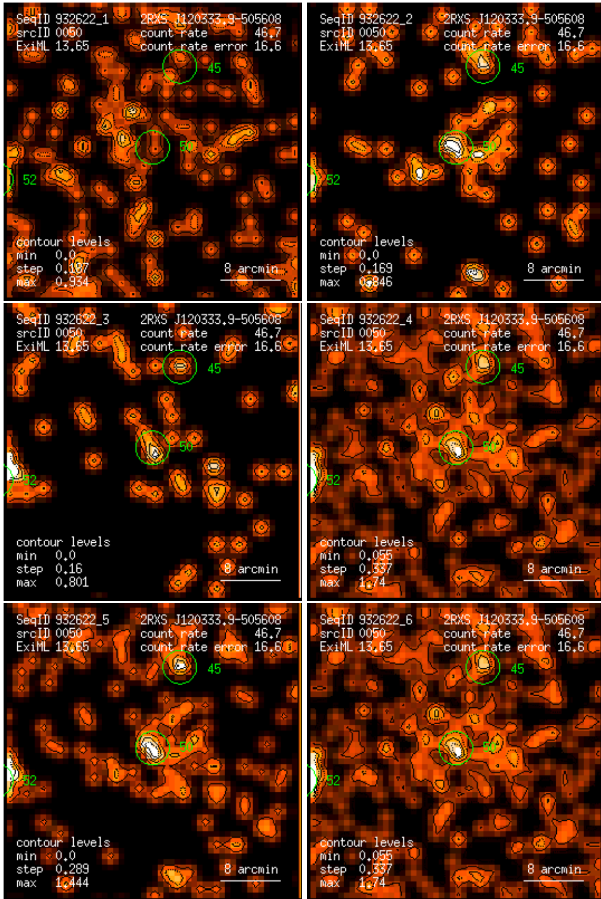
Figure 50: RASS 932622: detection 0050: band rate images, Gaussian filter: (1) PSPC channels 11 – 41, (2) 52 – 90, (3) 91 – 201, (4) 11 – 235, (5) 52 – 201, (6) 11 – 201. Broad band rates in counts/ks. Band rate contour levels in counts/ks/arcmin 2 .
