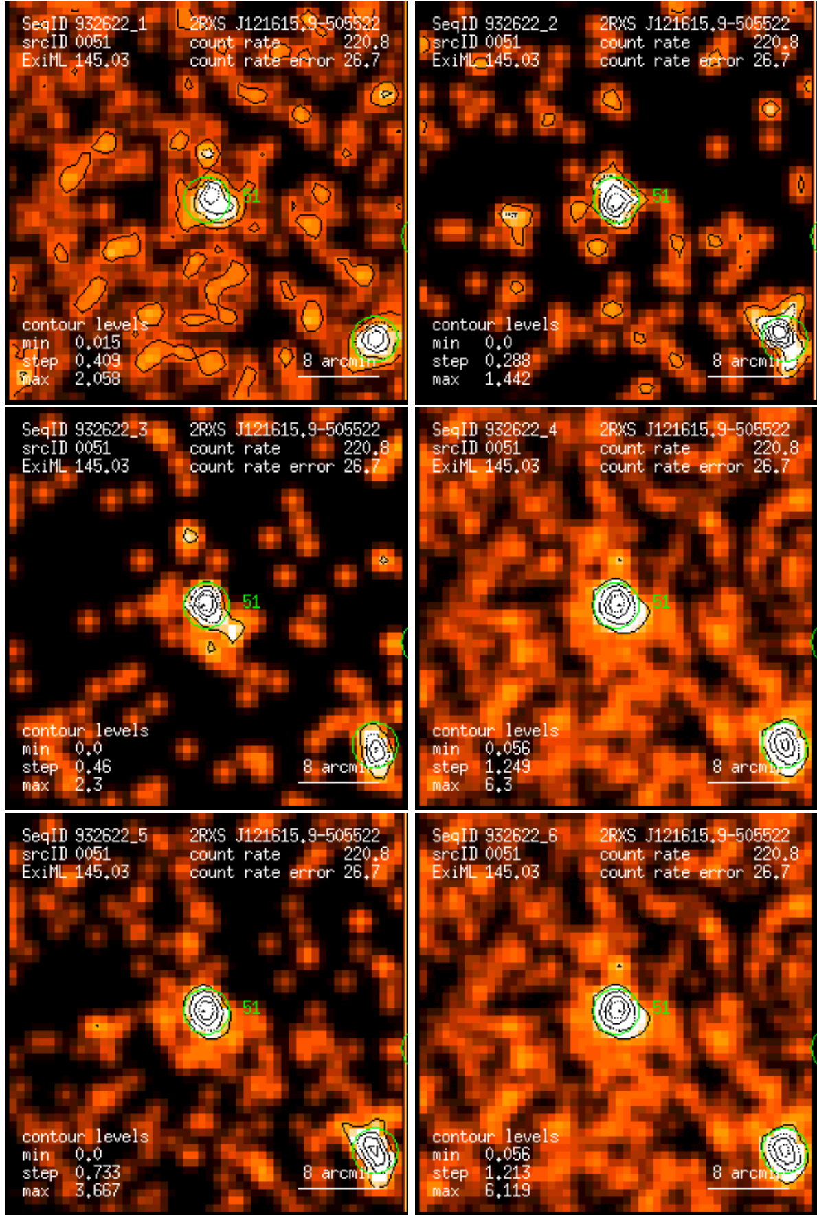
Figure 51: RASS 932622: detection 0051: band rate images, Gaussian filter: (1) PSPC channels 11 – 41, (2) 52 – 90, (3) 91 – 201, (4) 11 – 235, (5) 52 – 201, (6) 11 – 201. Broad band rates in counts/ks. Band rate contour levels in counts/ks/arcmin 2 .
