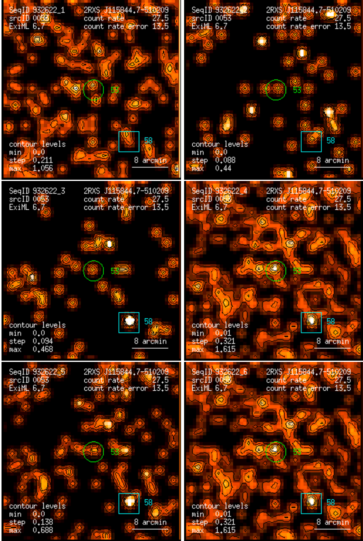
Figure 53: RASS 932622: detection 0053: band rate images, Gaussian filter: (1) PSPC channels 11 – 41, (2) 52 – 90, (3) 91 – 201, (4) 11 – 235, (5) 52 – 201, (6) 11 – 201. Broad band rates in counts/ks. Band rate contour levels in counts/ks/arcmin 2 .
