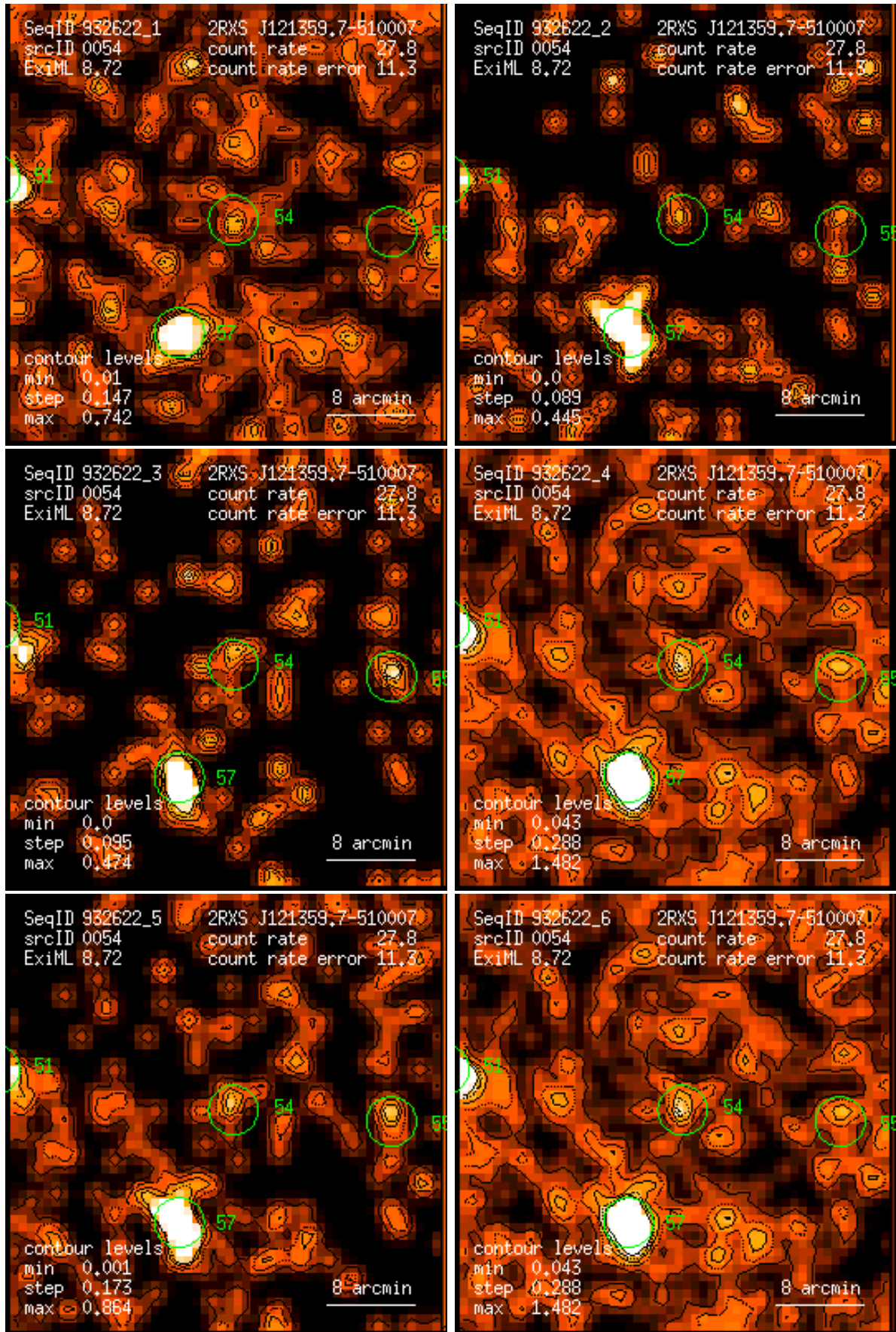
Figure 54: RASS 932622: detection 0054: band rate images, Gaussian filter: (1) PSPC channels 11 – 41, (2) 52 – 90, (3) 91 – 201, (4) 11 – 235, (5) 52 – 201, (6) 11 – 201. Broad band rates in counts/ks. Band rate contour levels in counts/ks/arcmin 2 .
