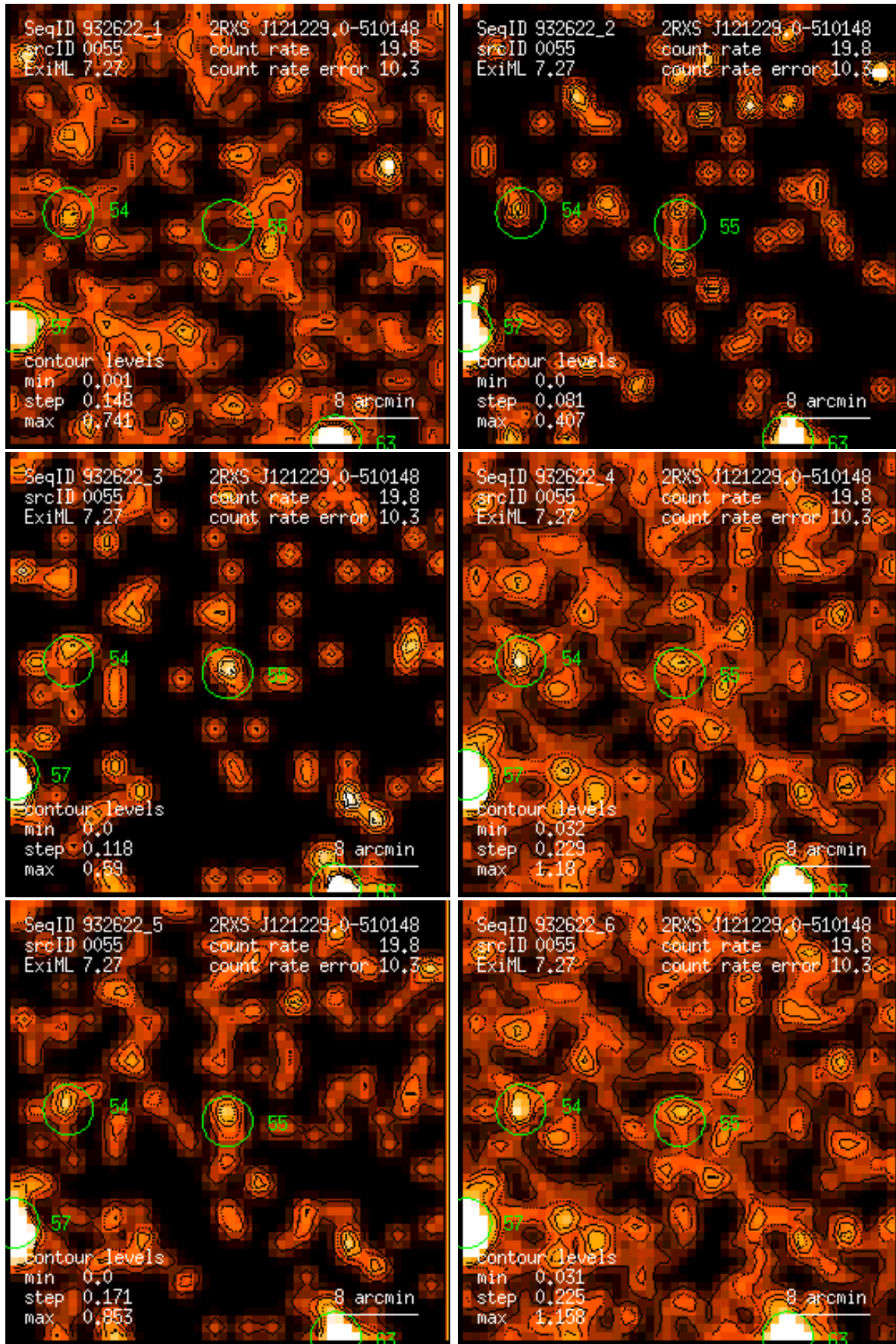
Figure 55: RASS 932622: detection 0055: band rate images, Gaussian filter: (1) PSPC channels 11 – 41, (2) 52 – 90, (3) 91 – 201, (4) 11 – 235, (5) 52 – 201, (6) 11 – 201. Broad band rates in counts/ks. Band rate contour levels in counts/ks/arcmin 2 .
