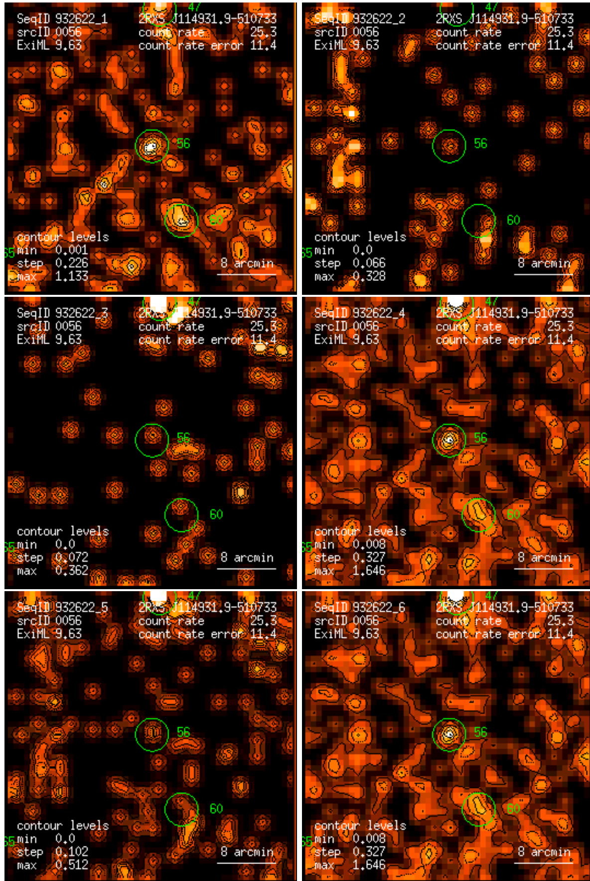
Figure 56: RASS 932622: detection 0056: band rate images, Gaussian filter: (1) PSPC channels 11 – 41, (2) 52 – 90, (3) 91 – 201, (4) 11 – 235, (5) 52 – 201, (6) 11 – 201. Broad band rates in counts/ks. Band rate contour levels in counts/ks/arcmin 2 .
