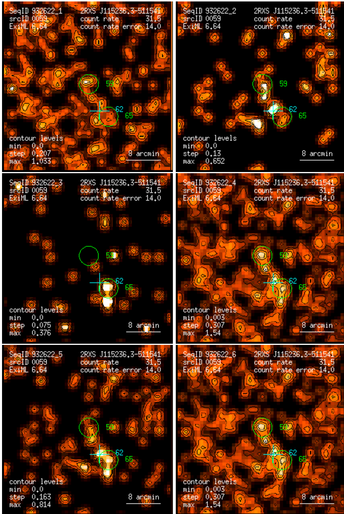
Figure 59: RASS 932622: detection 0059: band rate images, Gaussian filter: (1) PSPC channels 11 – 41, (2) 52 – 90, (3) 91 – 201, (4) 11 – 235, (5) 52 – 201, (6) 11 – 201. Broad band rates in counts/ks. Band rate contour levels in counts/ks/arcmin 2 .
