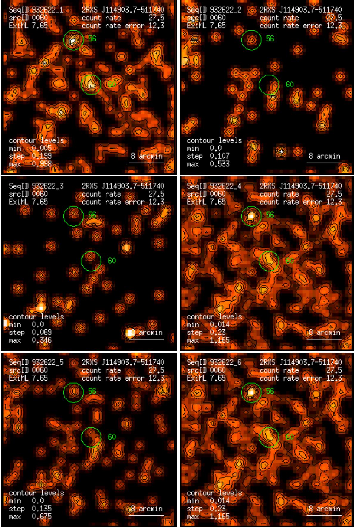
Figure 60: RASS 932622: detection 0060: band rate images, Gaussian filter: (1) PSPC channels 11 – 41, (2) 52 – 90, (3) 91 – 201, (4) 11 – 235, (5) 52 – 201, (6) 11 – 201. Broad band rates in counts/ks. Band rate contour levels in counts/ks/arcmin 2 .
