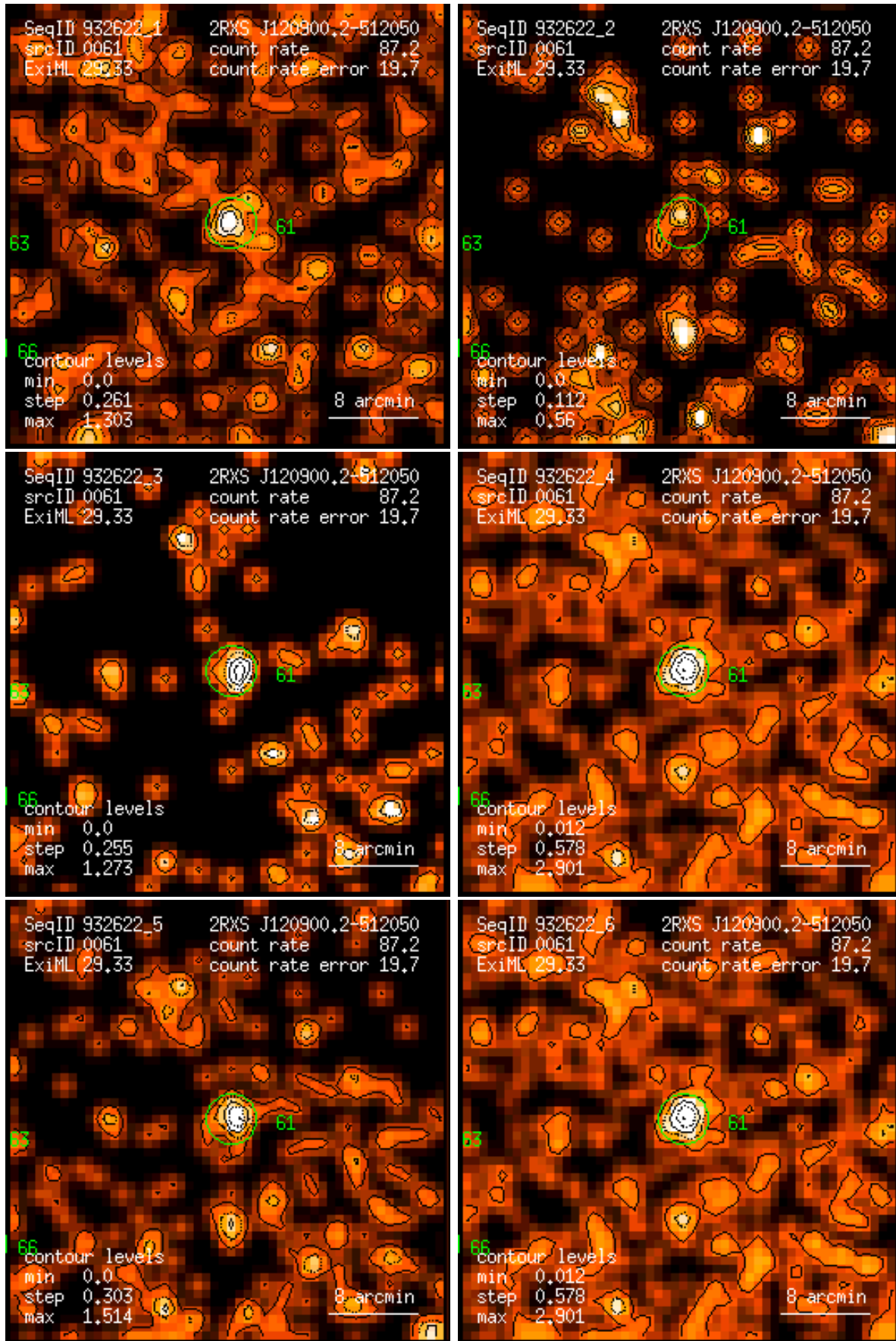
Figure 61: RASS 932622: detection 0061: band rate images, Gaussian filter: (1) PSPC channels 11 – 41, (2) 52 – 90, (3) 91 – 201, (4) 11 – 235, (5) 52 – 201, (6) 11 – 201. Broad band rates in counts/ks. Band rate contour levels in counts/ks/arcmin 2 .
