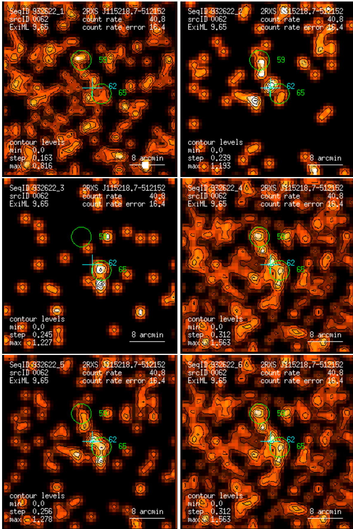
Figure 62: RASS 932622: detection 0062: band rate images, Gaussian filter: (1) PSPC channels 11 – 41, (2) 52 – 90, (3) 91 – 201, (4) 11 – 235, (5) 52 – 201, (6) 11 – 201. Broad band rates in counts/ks. Band rate contour levels in counts/ks/arcmin 2 .
