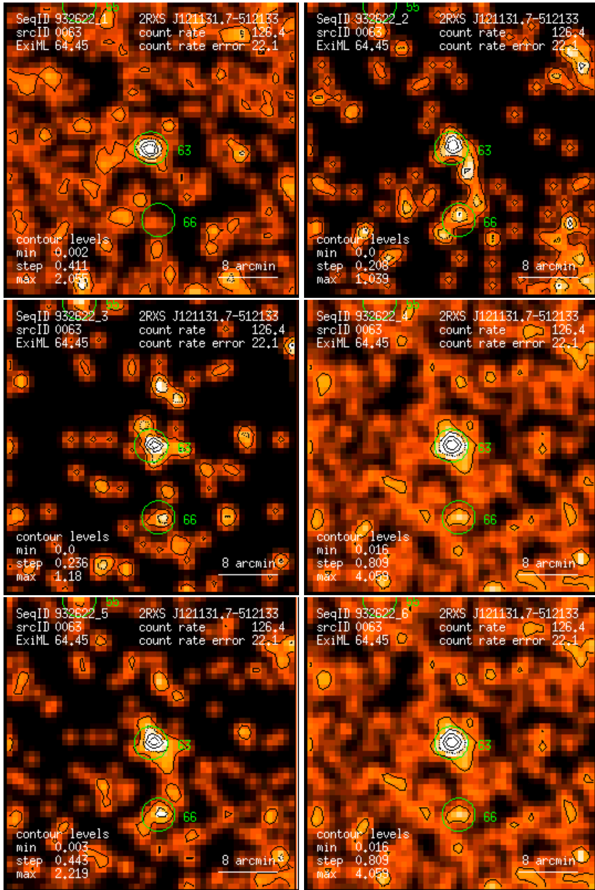
Figure 63: RASS 932622: detection 0063: band rate images, Gaussian filter: (1) PSPC channels 11 – 41, (2) 52 – 90, (3) 91 – 201, (4) 11 – 235, (5) 52 – 201, (6) 11 – 201. Broad band rates in counts/ks. Band rate contour levels in counts/ks/arcmin 2 .
