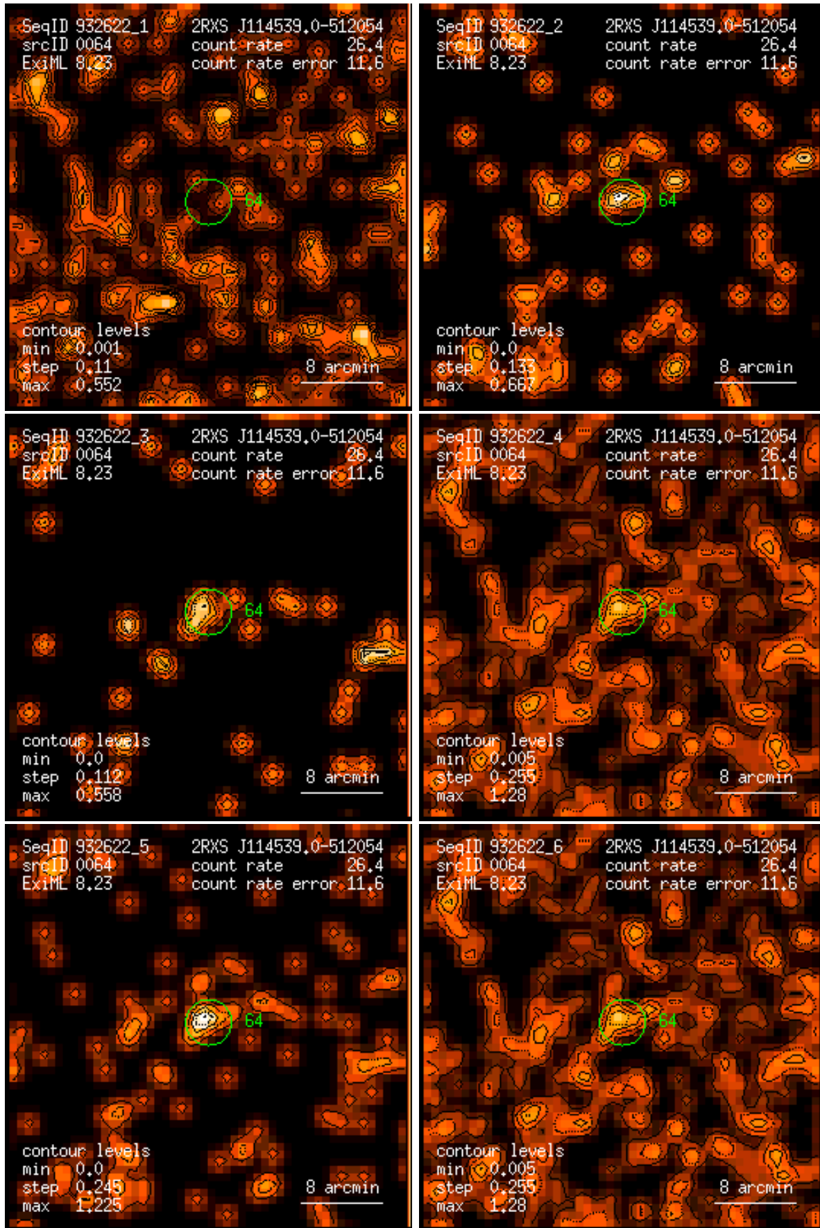
Figure 64: RASS 932622: detection 0064: band rate images, Gaussian filter: (1) PSPC channels 11 – 41, (2) 52 – 90, (3) 91 – 201, (4) 11 – 235, (5) 52 – 201, (6) 11 – 201. Broad band rates in counts/ks. Band rate contour levels in counts/ks/arcmin 2 .
