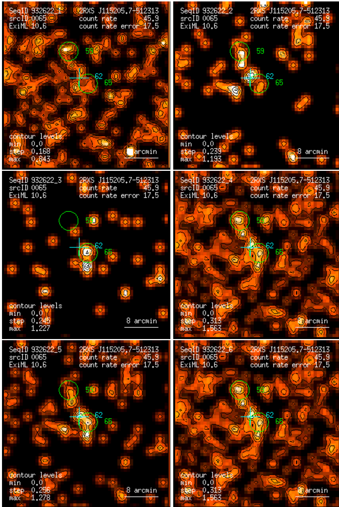
Figure 65: RASS 932622: detection 0065: band rate images, Gaussian filter: (1) PSPC channels 11 – 41, (2) 52 – 90, (3) 91 – 201, (4) 11 – 235, (5) 52 – 201, (6) 11 – 201. Broad band rates in counts/ks. Band rate contour levels in counts/ks/arcmin 2 .
