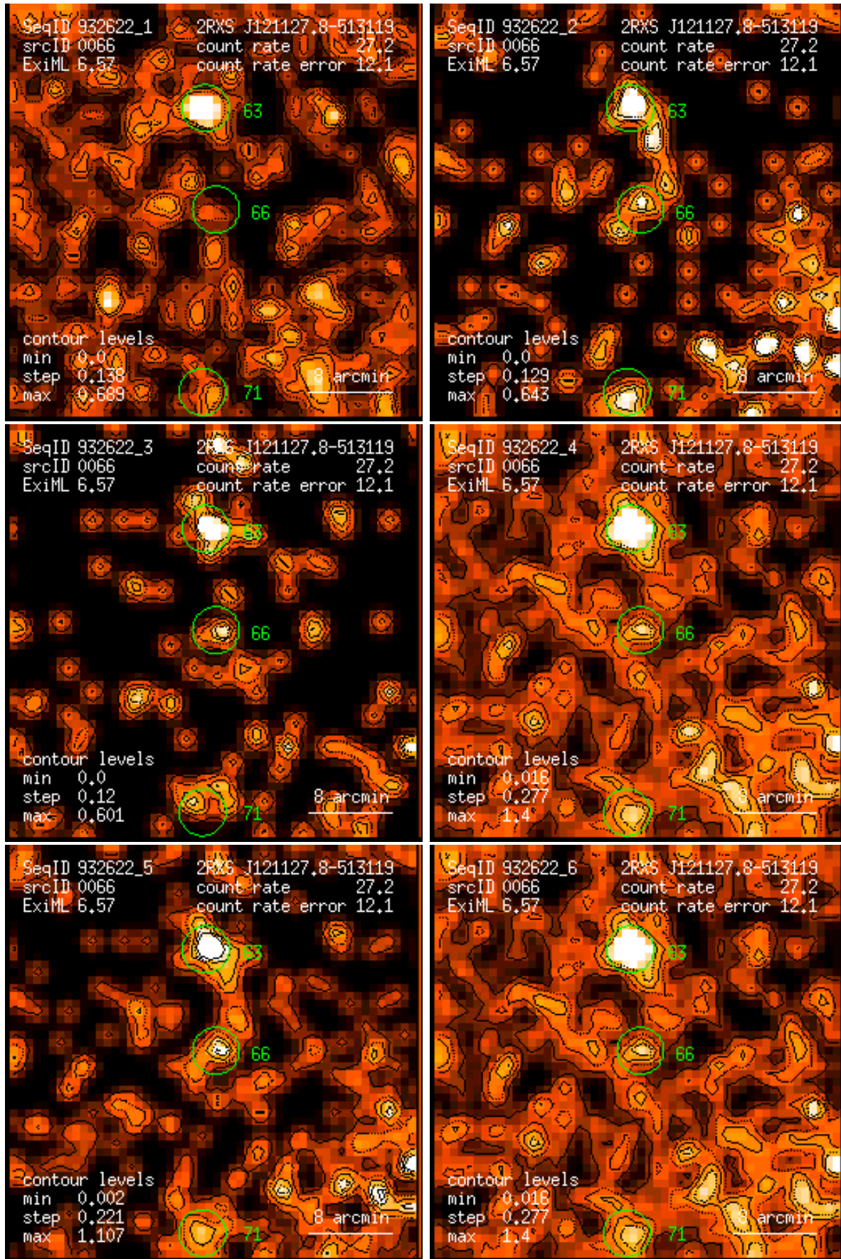
Figure 66: RASS 932622: detection 0066: band rate images, Gaussian filter: (1) PSPC channels 11 – 41, (2) 52 – 90, (3) 91 – 201, (4) 11 – 235, (5) 52 – 201, (6) 11 – 201. Broad band rates in counts/ks. Band rate contour levels in counts/ks/arcmin 2 .
