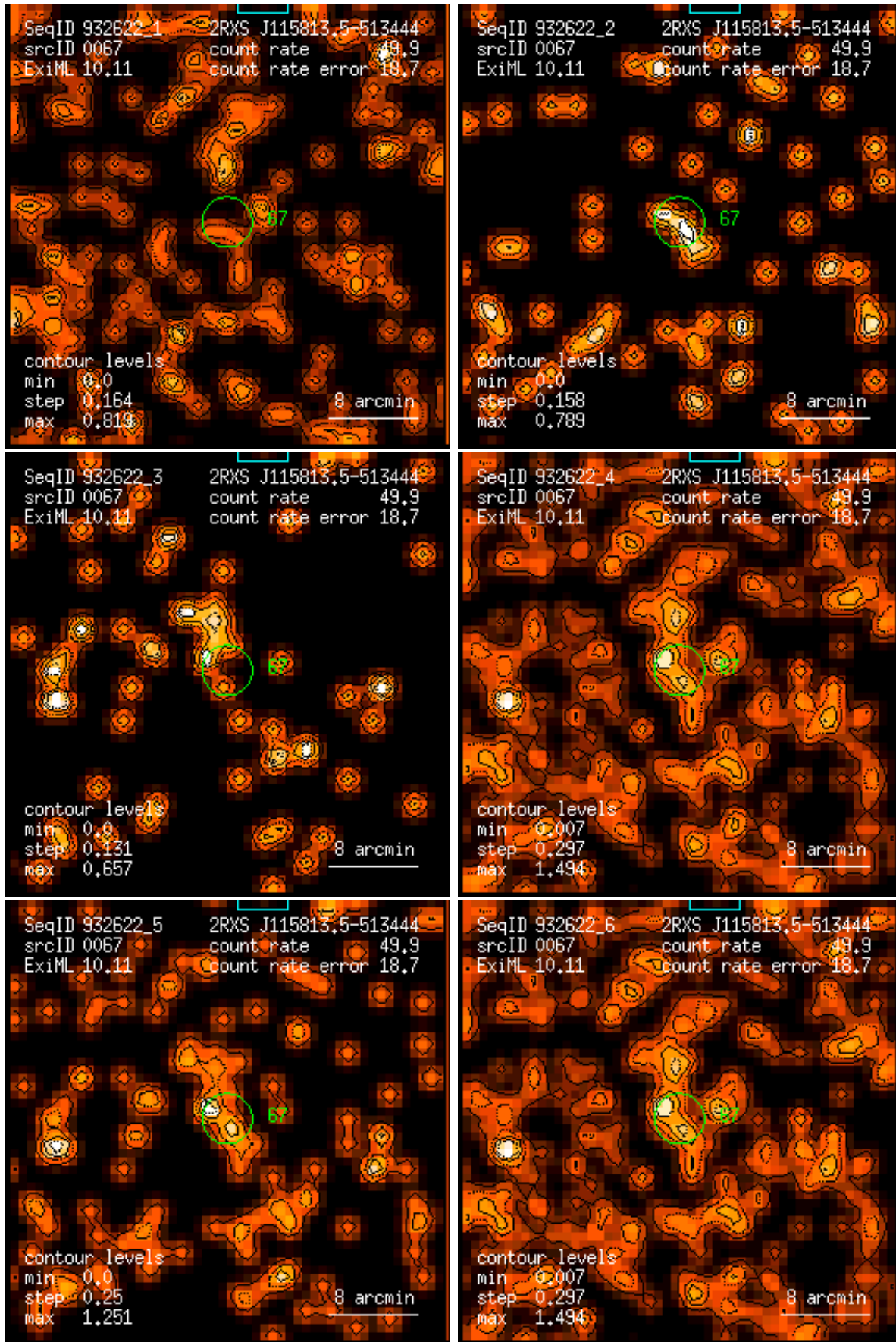
Figure 67: RASS 932622: detection 0067: band rate images, Gaussian filter: (1) PSPC channels 11 – 41, (2) 52 – 90, (3) 91 – 201, (4) 11 – 235, (5) 52 – 201, (6) 11 – 201. Broad band rates in counts/ks. Band rate contour levels in counts/ks/arcmin 2 .
