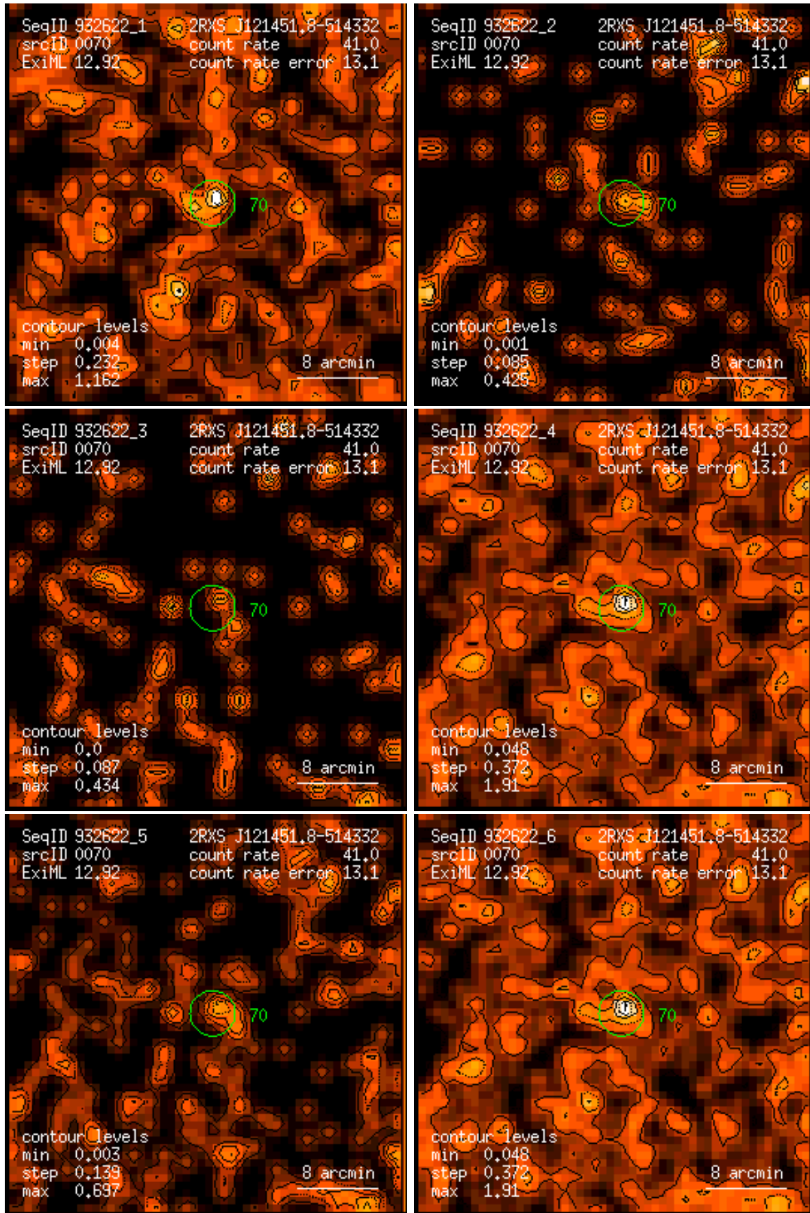
Figure 70: RASS 932622: detection 0070: band rate images, Gaussian filter: (1) PSPC channels 11 – 41, (2) 52 – 90, (3) 91 – 201, (4) 11 – 235, (5) 52 – 201, (6) 11 – 201. Broad band rates in counts/ks. Band rate contour levels in counts/ks/arcmin 2 .
