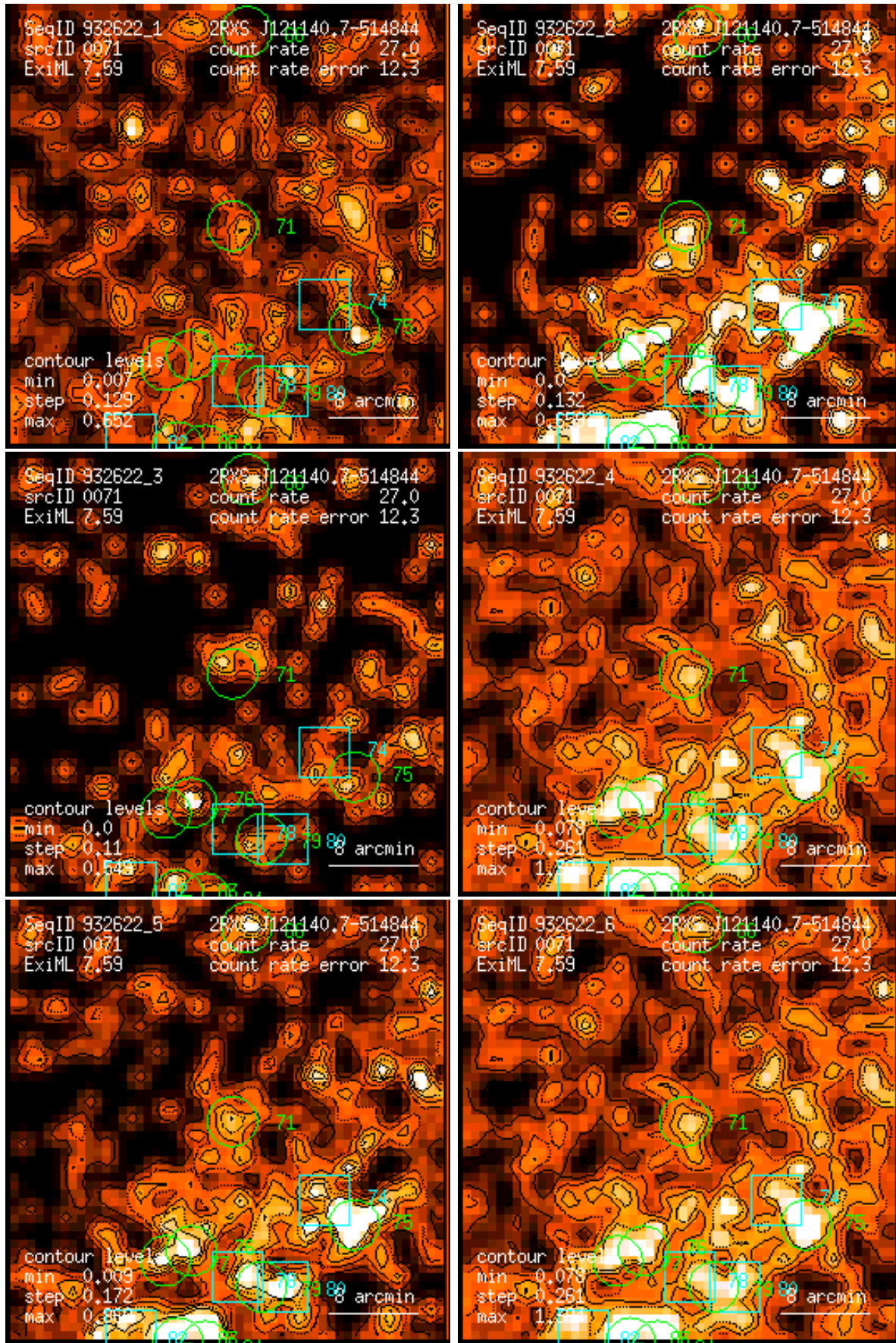
Figure 71: RASS 932622: detection 0071: band rate images, Gaussian filter: (1) PSPC channels 11 – 41, (2) 52 – 90, (3) 91 – 201, (4) 11 – 235, (5) 52 – 201, (6) 11 – 201. Broad band rates in counts/ks. Band rate contour levels in counts/ks/arcmin 2 .
