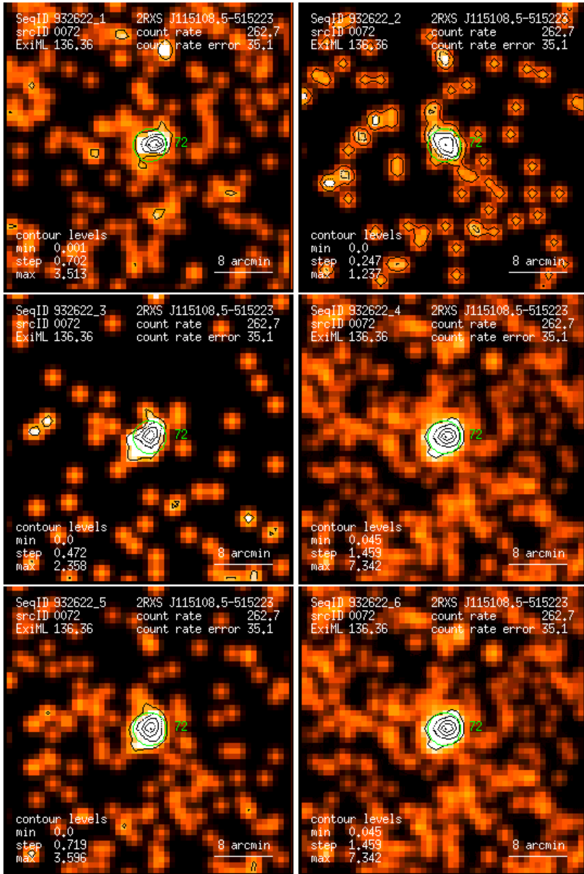
Figure 72: RASS 932622: detection 0072: band rate images, Gaussian filter: (1) PSPC channels 11 – 41, (2) 52 – 90, (3) 91 – 201, (4) 11 – 235, (5) 52 – 201, (6) 11 – 201. Broad band rates in counts/ks. Band rate contour levels in counts/ks/arcmin 2 .
