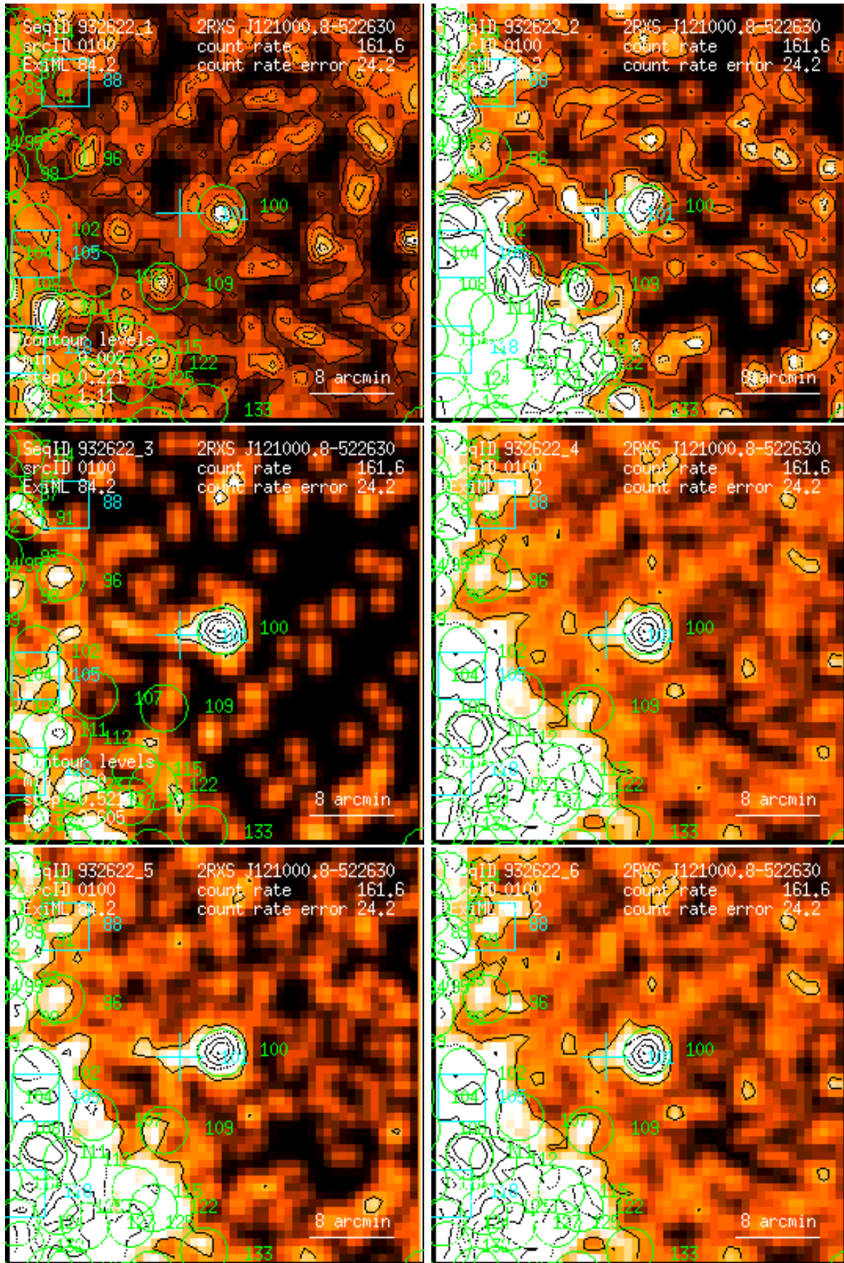
Figure 100: RASS 932622: detection 0100: band rate images, Gaussian filter: (1) PSPC channels 11 – 41, (2) 52 – 90, (3) 91 – 201, (4) 11 – 235, (5) 52 – 201, (6) 11 – 201. Broad band rates in counts/ks. Band rate contour levels in counts/ks/arcmin 2 .
