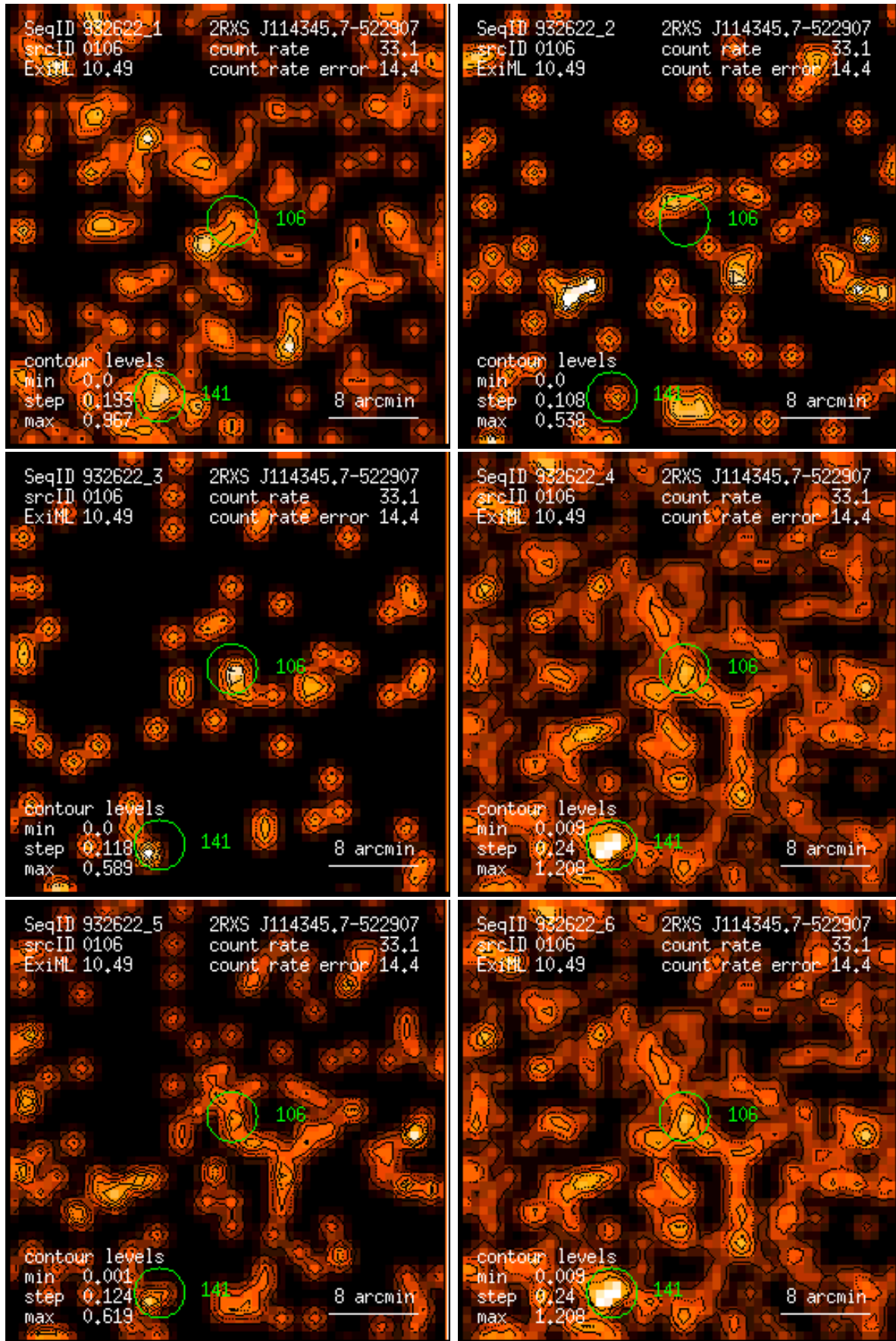
Figure 106: RASS 932622: detection 0106: band rate images, Gaussian filter: (1) PSPC channels 11 – 41, (2) 52 – 90, (3) 91 – 201, (4) 11 – 235, (5) 52 – 201, (6) 11 – 201. Broad band rates in counts/ks. Band rate contour levels in counts/ks/arcmin 2 .
