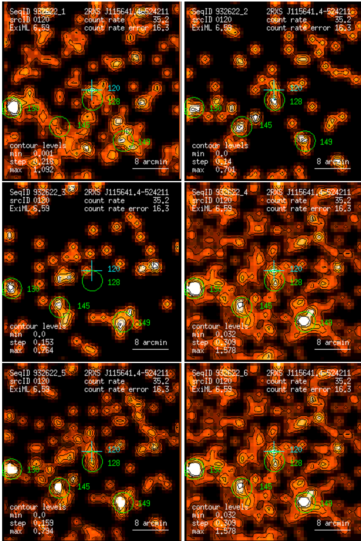
Figure 120: RASS 932622: detection 0120: band rate images, Gaussian filter: (1) PSPC channels 11 – 41, (2) 52 – 90, (3) 91 – 201, (4) 11 – 235, (5) 52 – 201, (6) 11 – 201. Broad band rates in counts/ks. Band rate contour levels in counts/ks/arcmin 2 .
