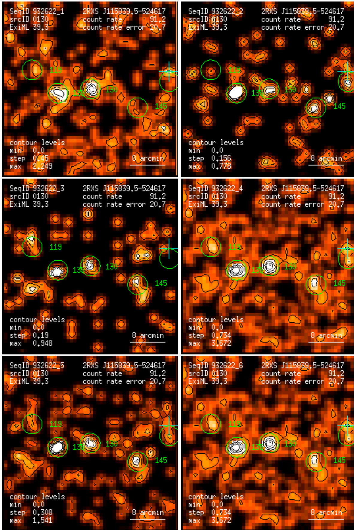
Figure 130: RASS 932622: detection 0130: band rate images, Gaussian filter: (1) PSPC channels 11 – 41, (2) 52 – 90, (3) 91 – 201, (4) 11 – 235, (5) 52 – 201, (6) 11 – 201. Broad band rates in counts/ks. Band rate contour levels in counts/ks/arcmin 2 .
