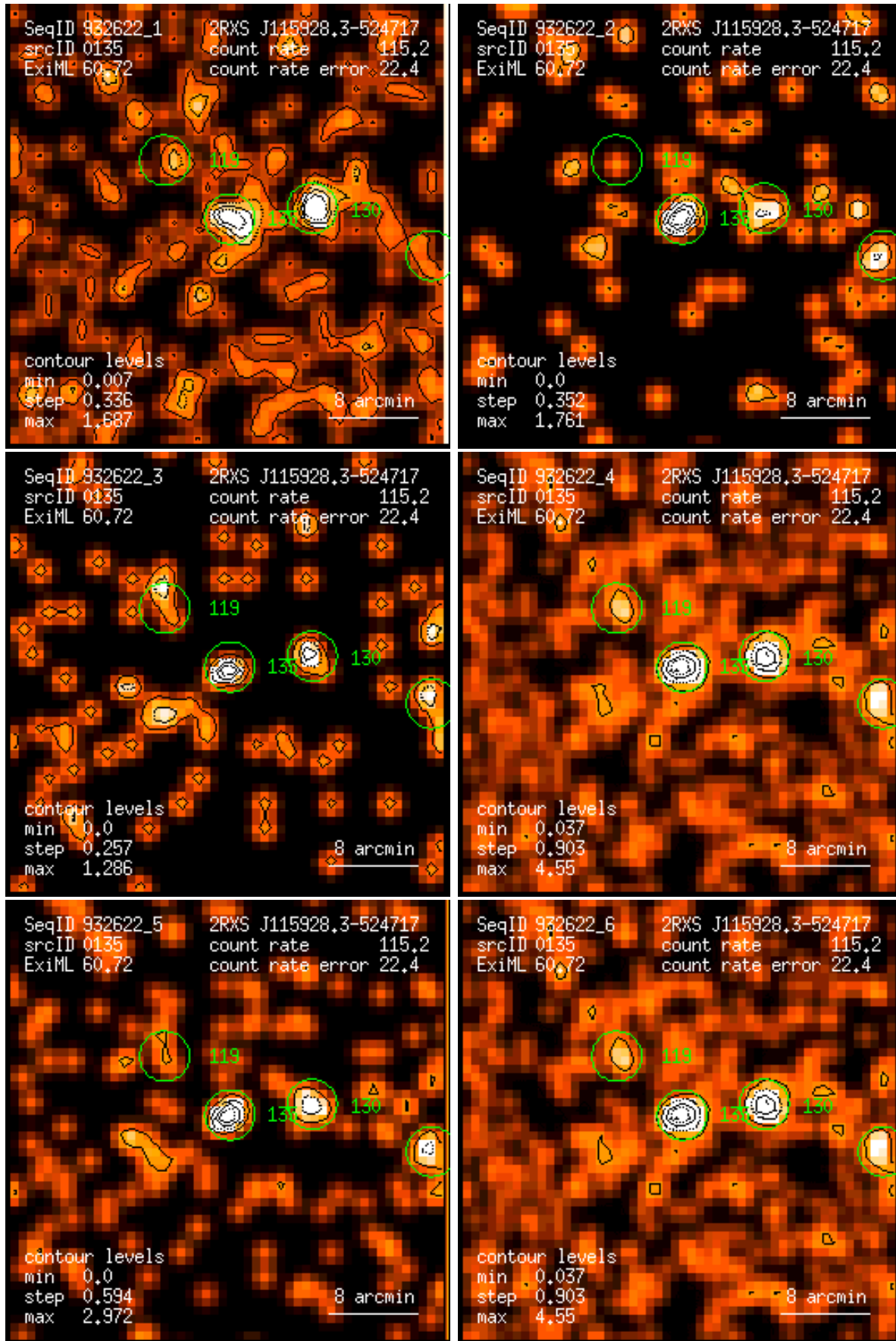
Figure 135: RASS 932622: detection 0135: band rate images, Gaussian filter: (1) PSPC channels 11 – 41, (2) 52 – 90, (3) 91 – 201, (4) 11 – 235, (5) 52 – 201, (6) 11 – 201. Broad band rates in counts/ks. Band rate contour levels in counts/ks/arcmin 2 .
