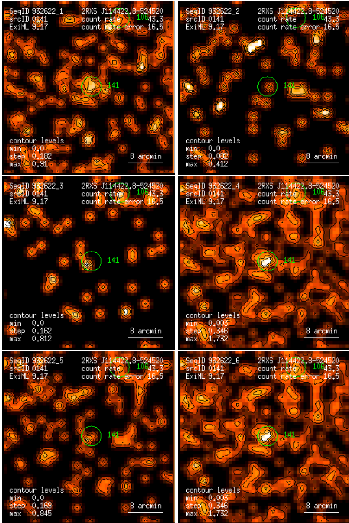
Figure 141: RASS 932622: detection 0141: band rate images, Gaussian filter: (1) PSPC channels 11 – 41, (2) 52 – 90, (3) 91 – 201, (4) 11 – 235, (5) 52 – 201, (6) 11 – 201. Broad band rates in counts/ks. Band rate contour levels in counts/ks/arcmin 2 .
