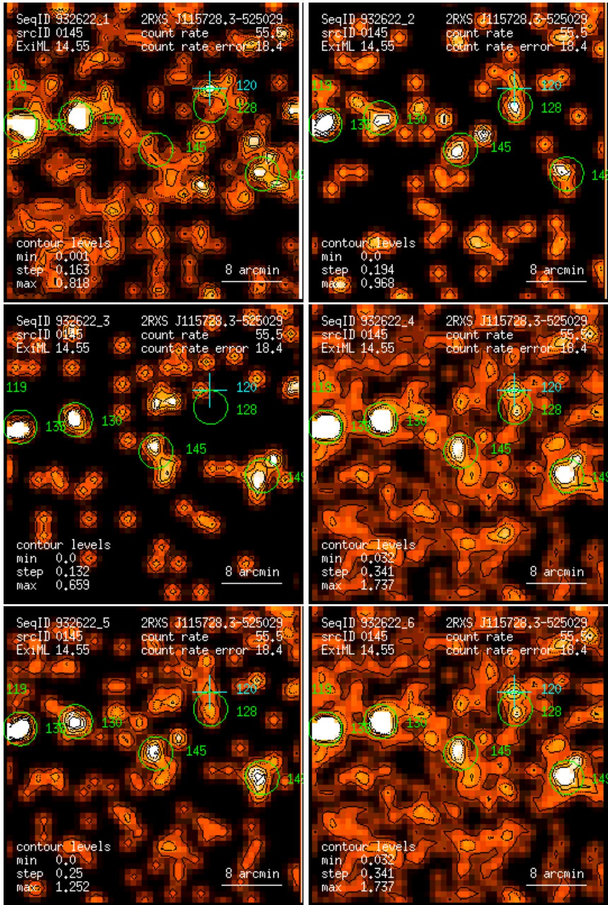
Figure 145: RASS 932622: detection 0145: band rate images, Gaussian filter: (1) PSPC channels 11 – 41, (2) 52 – 90, (3) 91 – 201, (4) 11 – 235, (5) 52 – 201, (6) 11 – 201. Broad band rates in counts/ks. Band rate contour levels in counts/ks/arcmin 2 .
